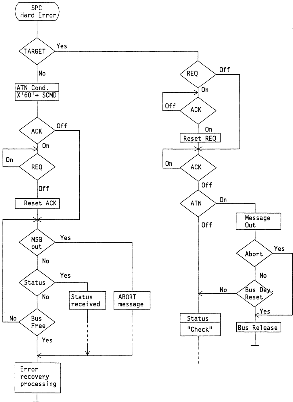
Fig. 4.11.4 Example of control processing for SPC-detected error (2)
