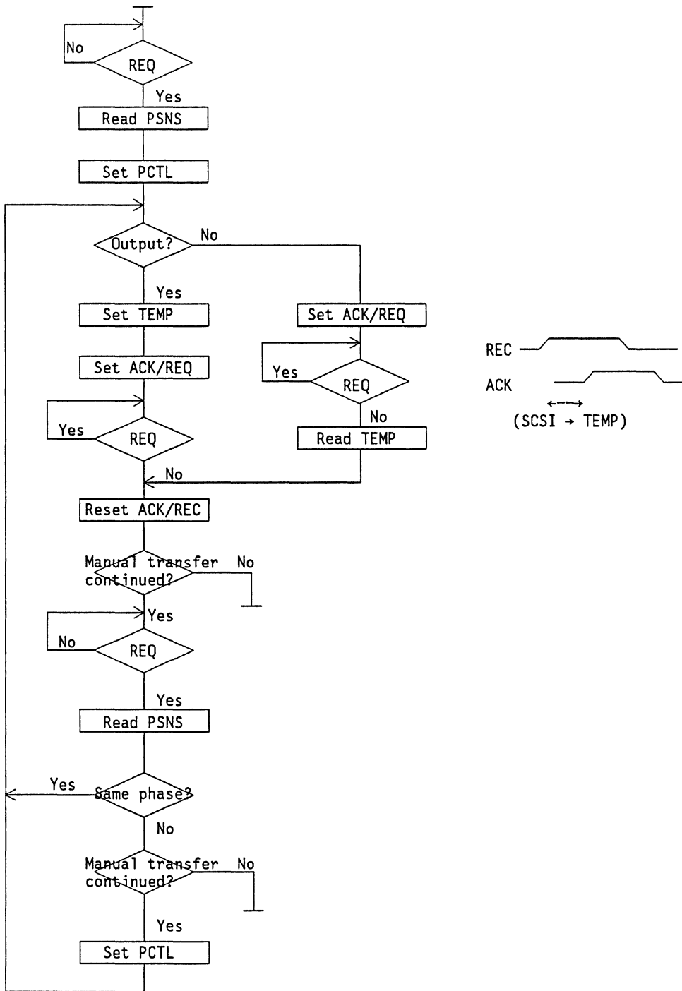
Fig. 4.3.5 Manual transfer procedure (SPC serving as an INITIATOR)
