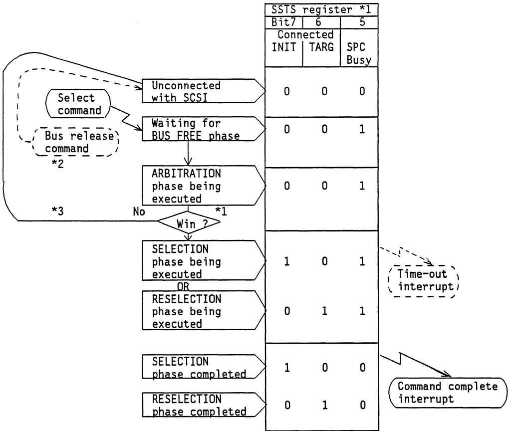
Fig. 4.3.1 Status transitions in Select command execution
