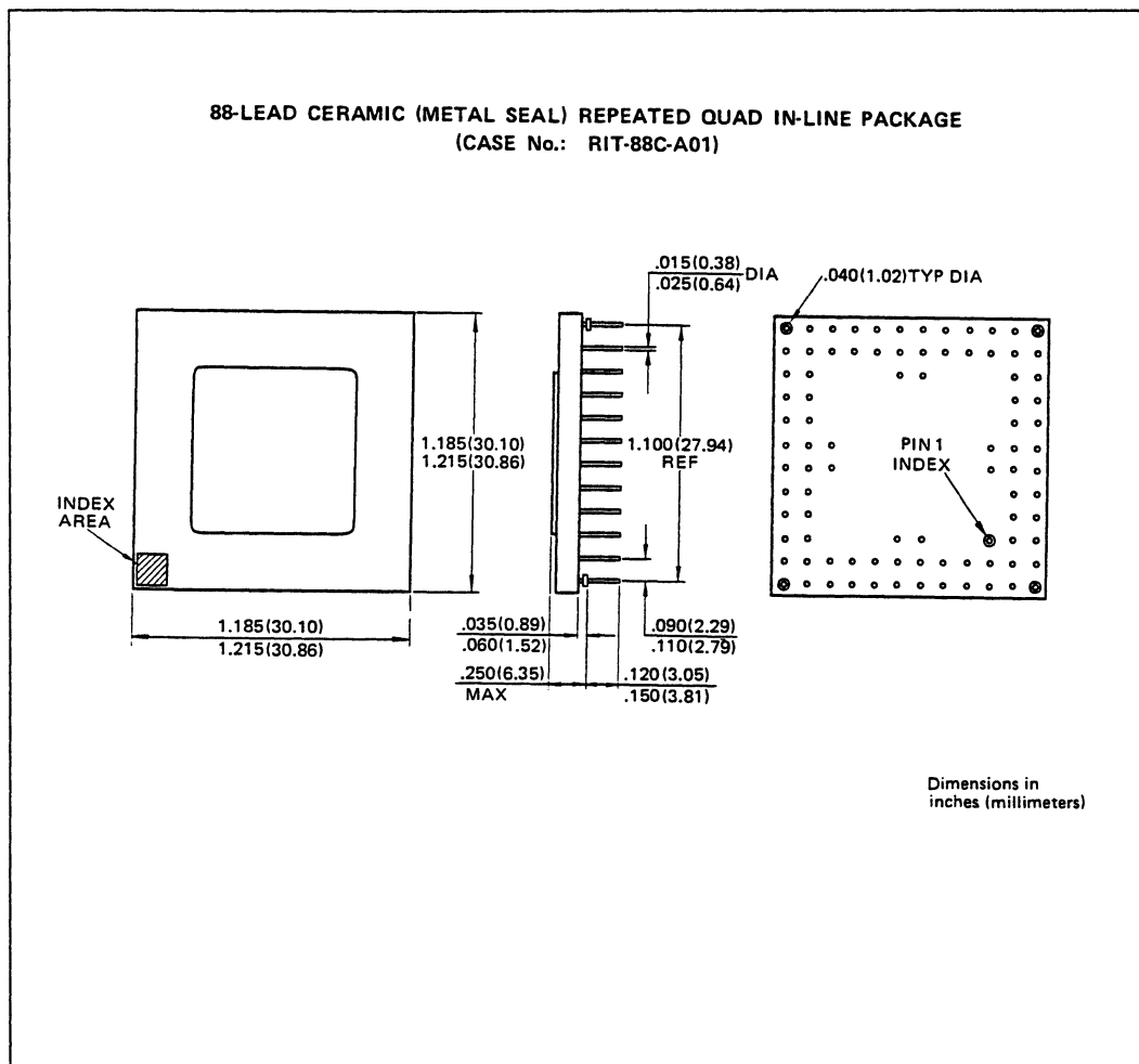
Figure 1.4.1 Dimensions of Package
