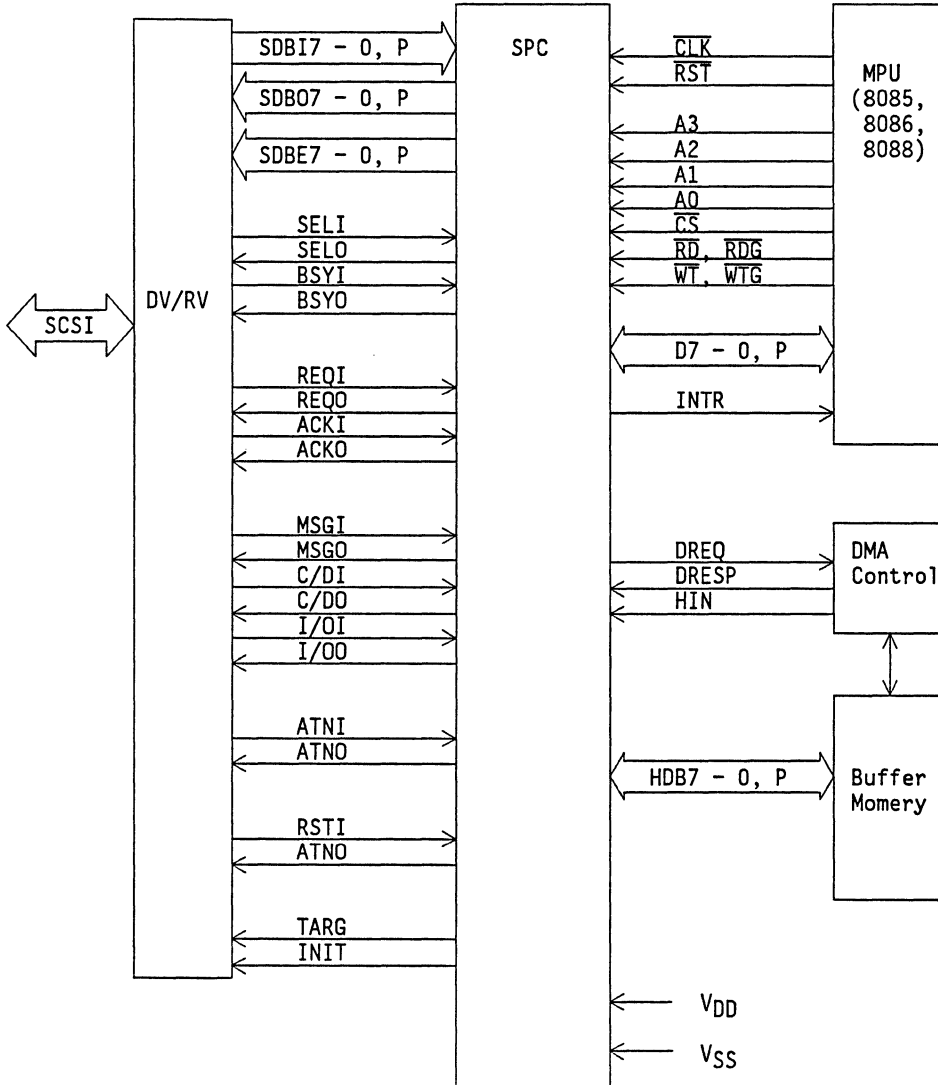
Fig. 5.1.1 Examples of external circuit connections
