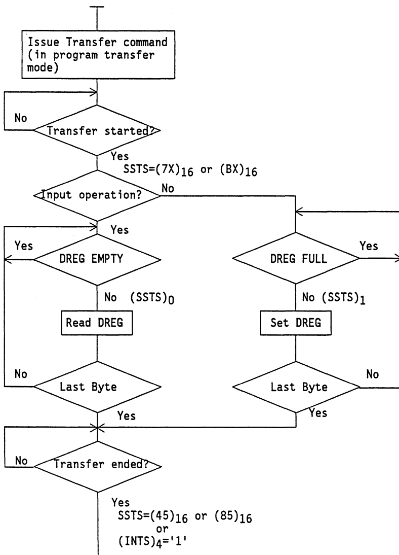
Fig. 4.6.1 DREG access procedure in program transfer mode
