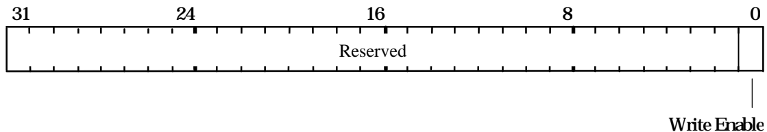
Figure 5.13 LBWriteMode Register
