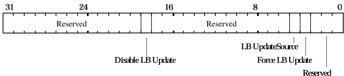
Figure 5.20 Window Register
