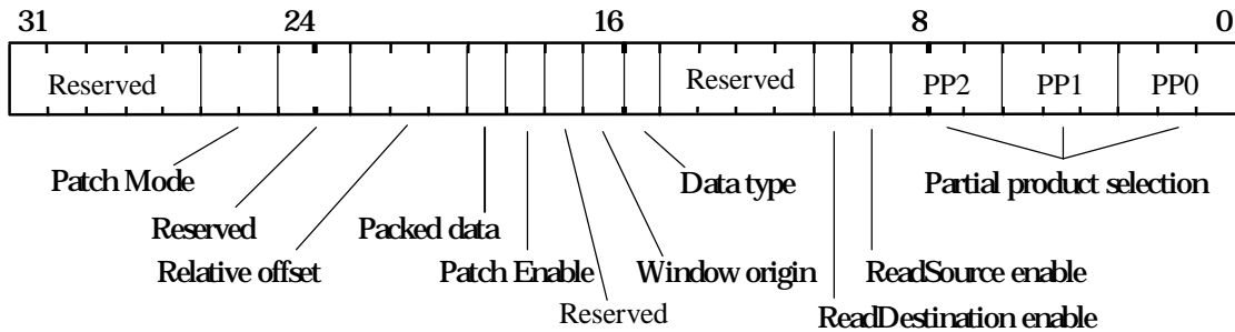
Figure 5.33 FBReadMode Register
