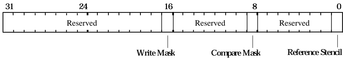
Figure 5.18 StencilData Register
