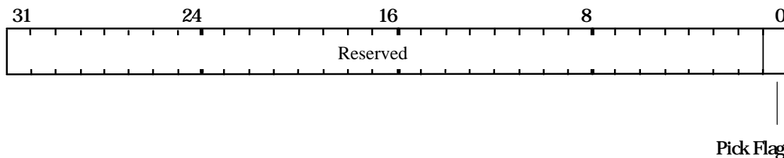
Figure 5.52 PickResult Register
