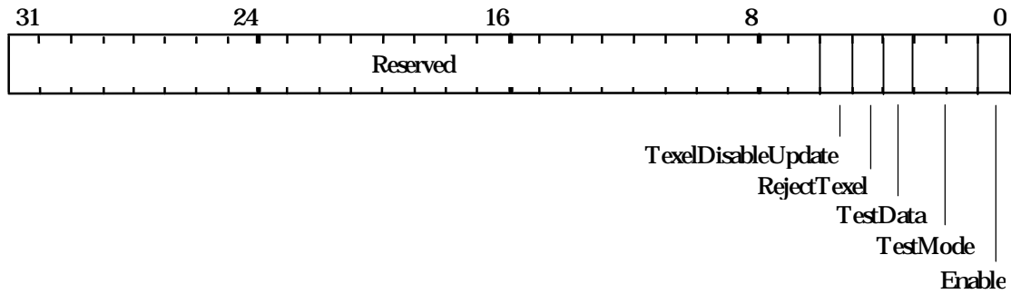
Figure 5.30 YUVMode Register
