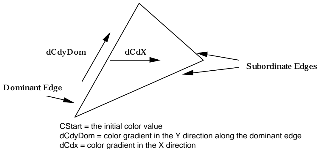
Figure 5.38 Color Interpolation
