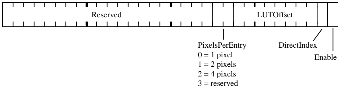
Figure 5.28 TexelLUTMode Register
