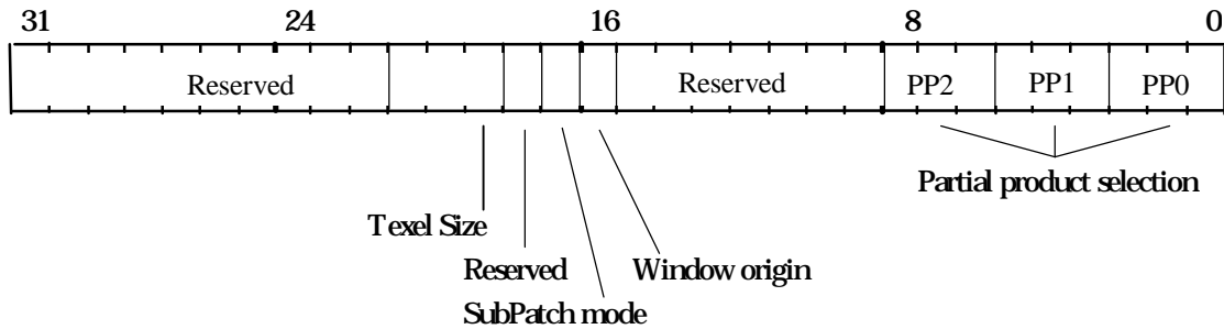
Figure 5.26 TextureMapFormat Register
