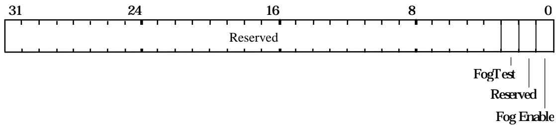
Figure 5.46 FogMode Register
