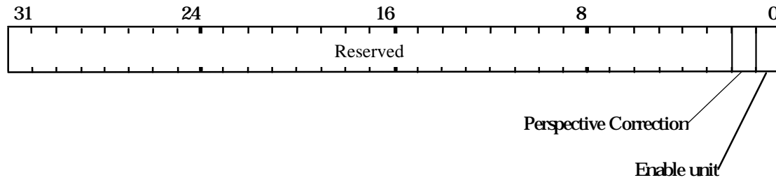
Figure 5.24 TextureAddressMode
