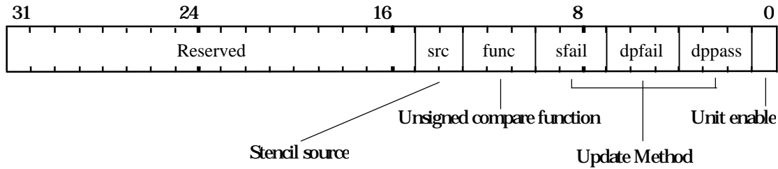
Figure 5.17 StencilMode Register
