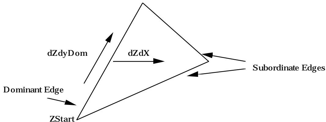
Figure 5.15 Depth Interpolation
