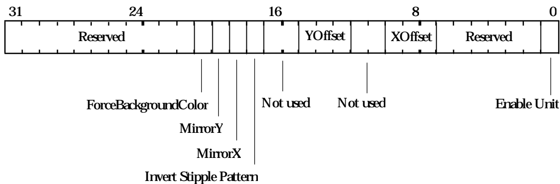
Figure 5.11 AreaStippleMode Register
