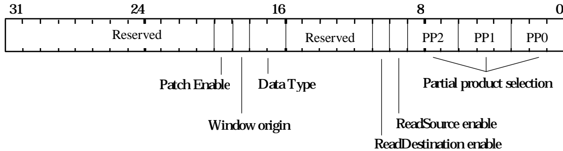
Figure 5.12 LBReadMode Register
