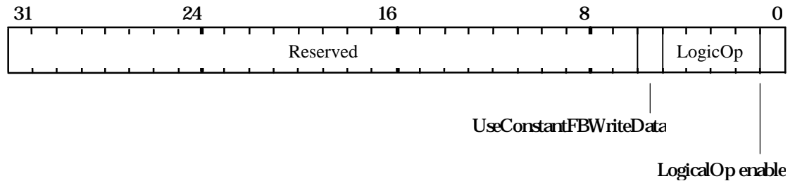
Figure 5.49 LogicalOpMode Register
