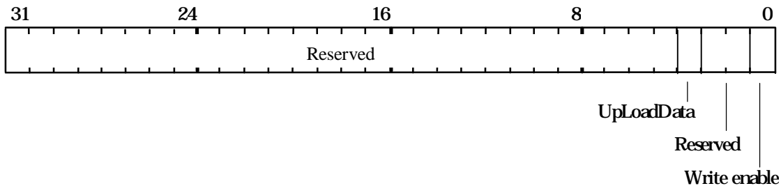
Figure 5.34 FBWriteMode Register
