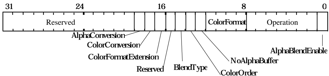
Figure 5.47 AlphaBlendMode Register
