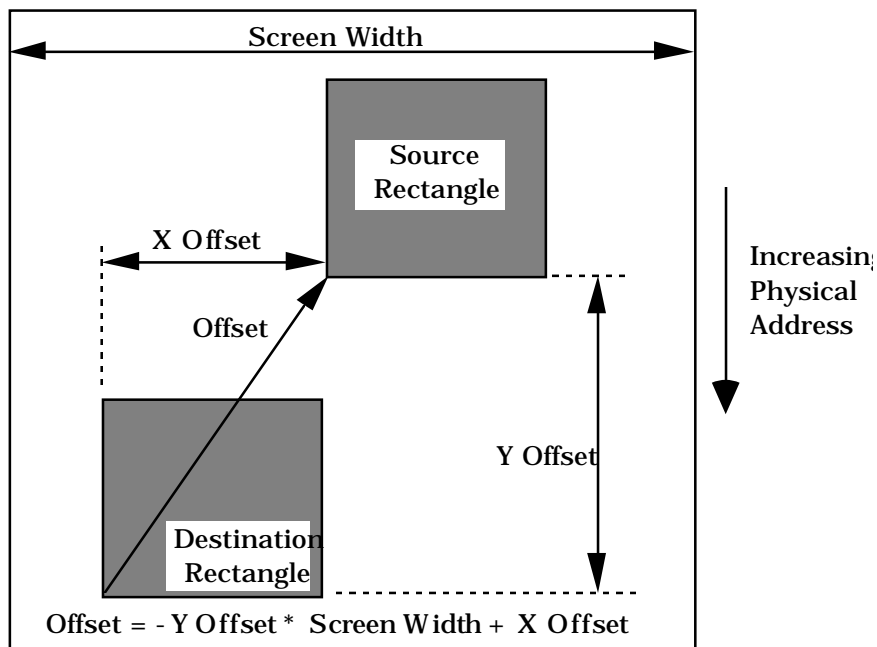
Figure 5.7 Copy Operation
