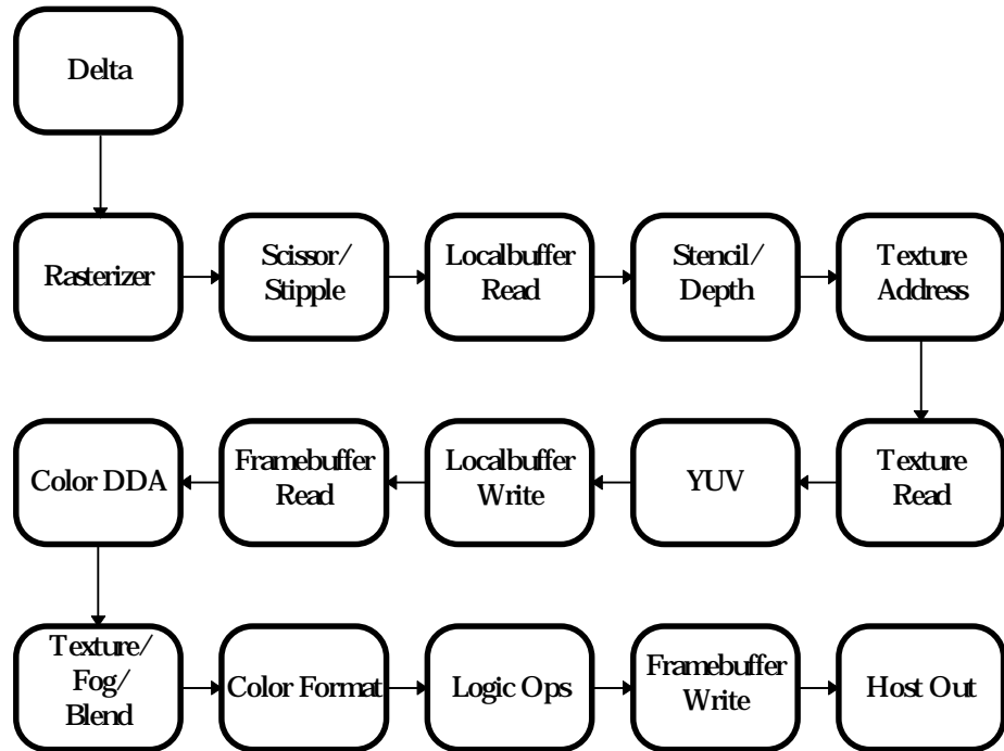
Figure 5.1 Hyperpipeline
