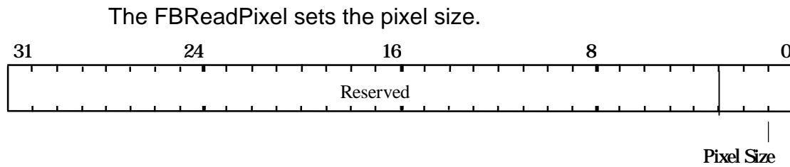
Figure 5.35 FBReadPixel Register
