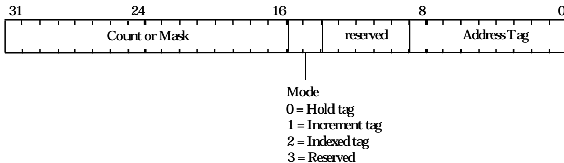
Figure 3.1 DMA Tag Description Format
