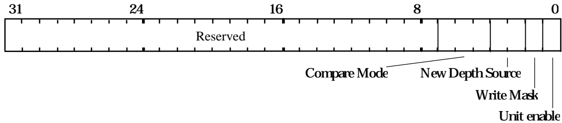
Figure 5.19 DepthMode Register
