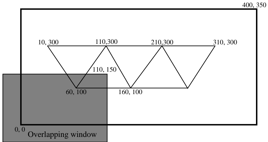
Figure 8.1 Geometry of the Mesh and Clip regions.
