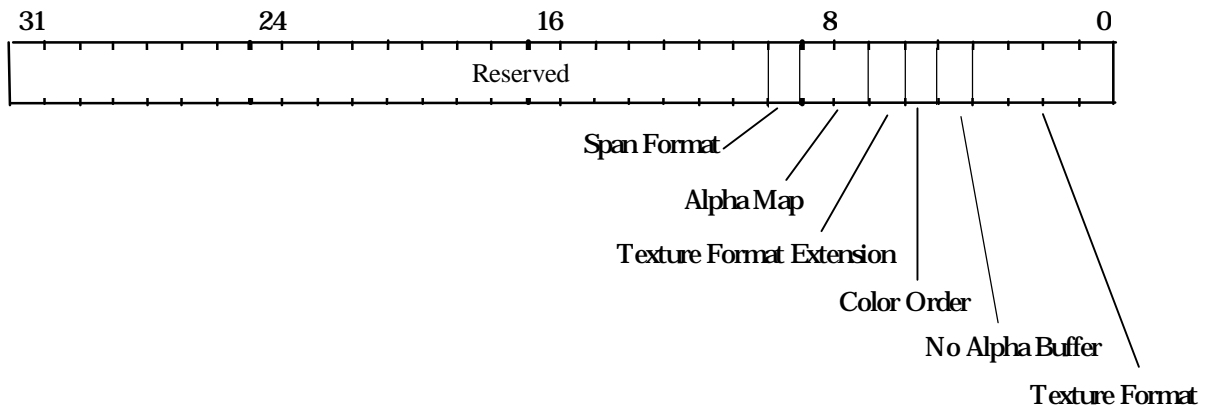
Figure 5.27 TextureDataFormat Register
