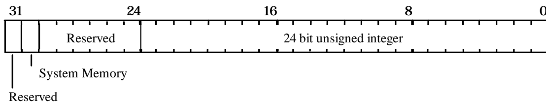
Figure 5.29 TexelLUTAddress register
