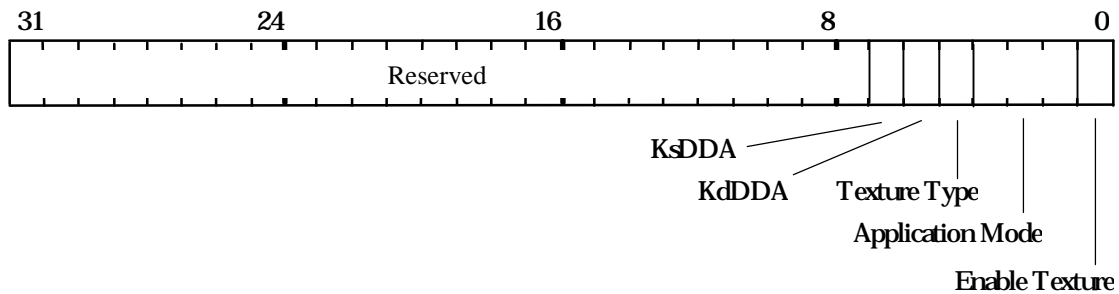
Figure 5.44 TextureColorMode Register
