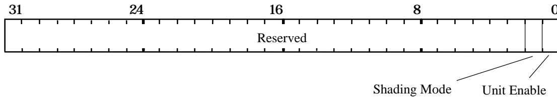
Figure 5.40 ColorDDAMode Register
