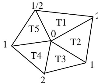
Figure 5.3 Triangle Fan.
