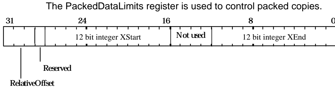
Figure 5.36 PackedDataLimits Register
