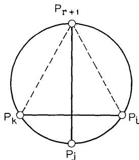
Fig. 10 — Configuration forbidden by hypothesis of Theorem 4. Dashed lines show edges of \bar{G} ; solid lines show edges of G .
