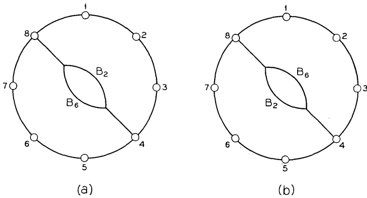
Fig. 19 — Proof of counterexample.
