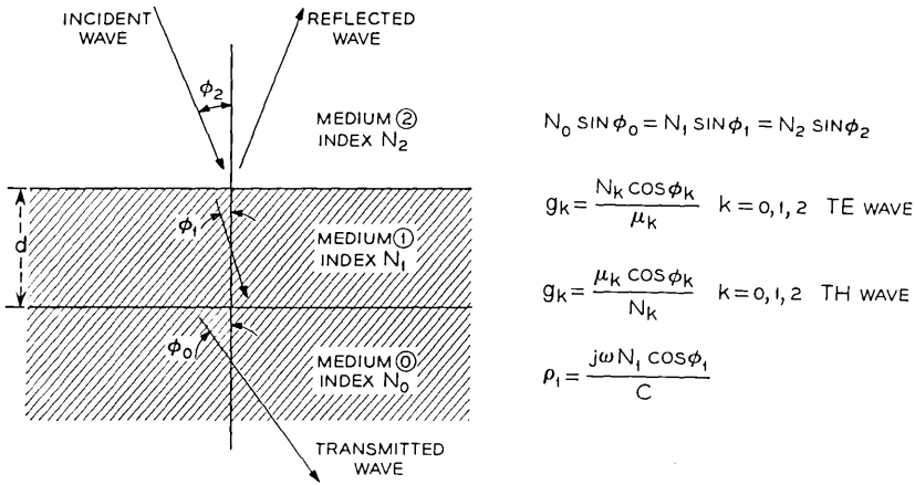
Fig. 9 — Reflection and transmission for 3 media.
