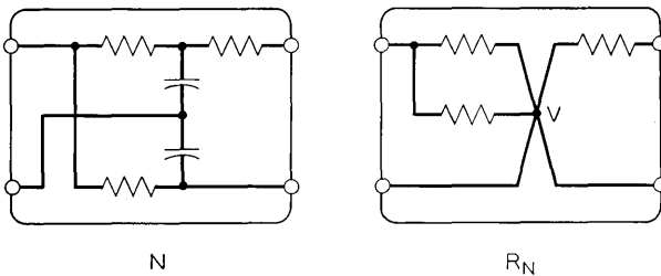
Fig. 3 — Nonplanar RC network N and reduced purely resistive network R_N .
