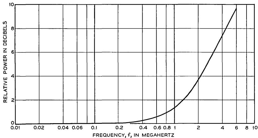
Fig. 5.—Pre-emphasis characteristic of a typical radio system.
