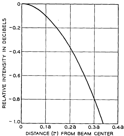
Fig. 8—Intensity distribution of Gaussian curve.
