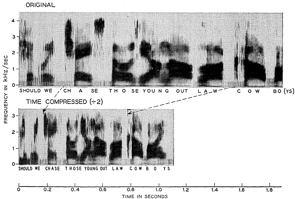
Fig. 8—Time compression of speech by a factor of 2. Male speaker A. (a) Original input; (b) Time-compressed output.
