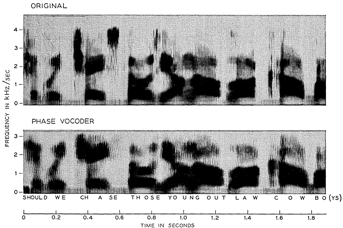
Fig. 6 — Spectrograms illustrating speech transmitted by the phase vocoder ( N = 30 ). The band-pass analysis is by sixth-order Bessel filters of 100-Hz band-width. Low-pass filtering of |F_n| and \varphi_n is by fourth-order Bessel filters with 25 Hz cut-off. Male speaker A. "Should we chase those young outlaw cowboys."
