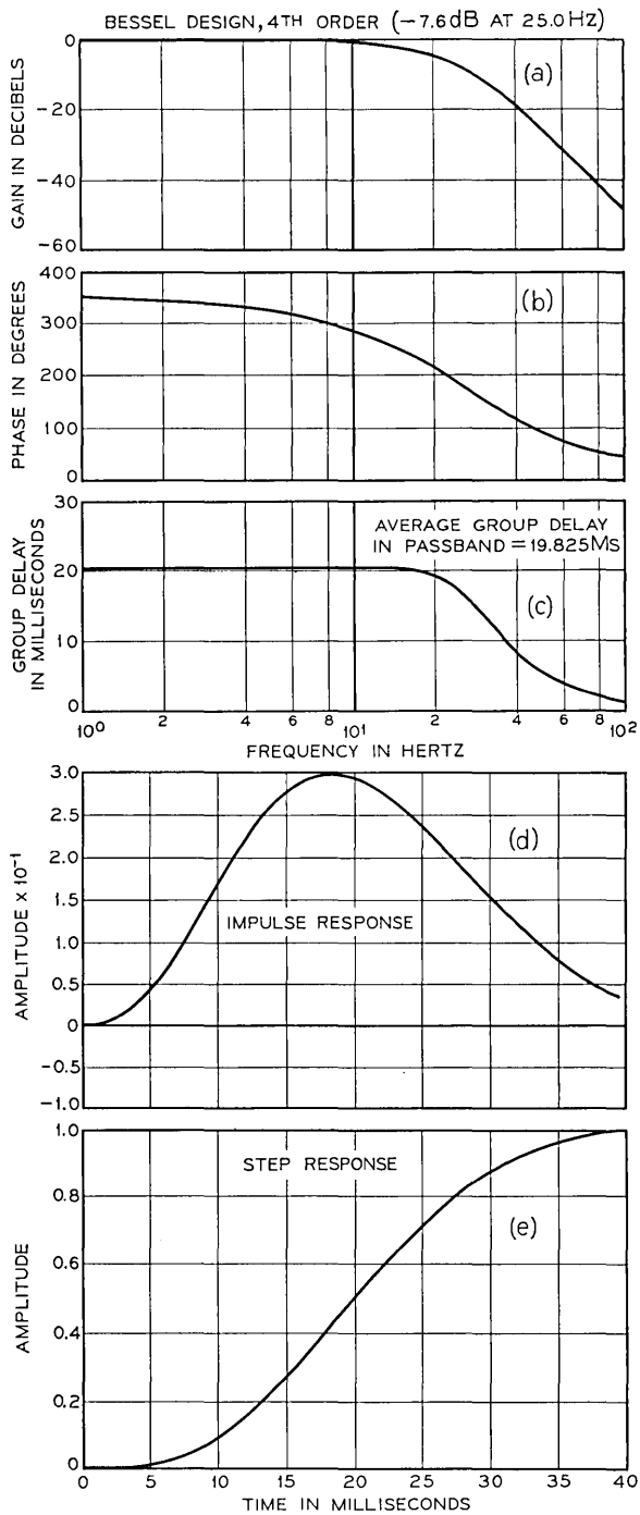
Fig. 5 — Fourth-order Bessel low-pass filter used to smooth the |F_n| and \dot{\varphi}_n signals.
