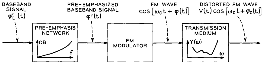
Fig. 1—Block diagram of a portion of an FM system.
