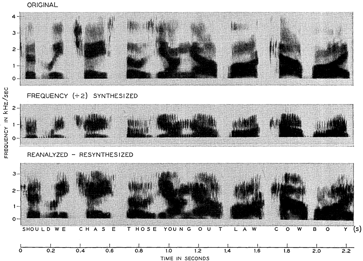
Fig. 7 — Self-multiplexing transmission for a bandwidth reduction of 2:1. (a) Original input; (b) Frequency-divided synthetic signal for analog transmission over one-half bandwidth channel; (c) Synthesized output from the reanalyzed, frequency-multiplied, half-band signal. Male speaker B.
