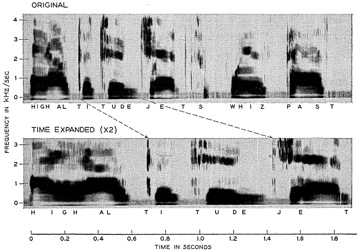
Fig. 9 — Time expansion of speech by a factor of 2. Female speaker. “High altitude jets whiz past screaming.” (a) Original input; (b) Time-expanded output.
