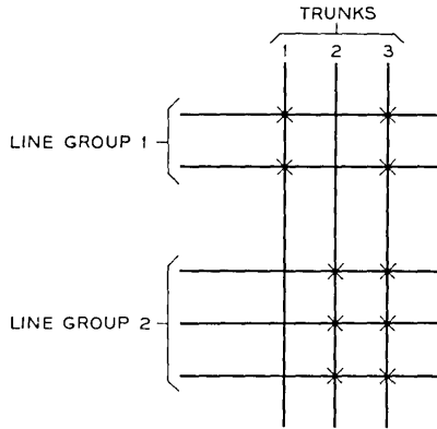
Fig. 13 — Second asymmetric grading.
