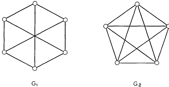
Fig. 7 — Kuratowski graphs.
