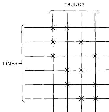
Fig. 3 — 6-to-4, 2 access concentrator.
