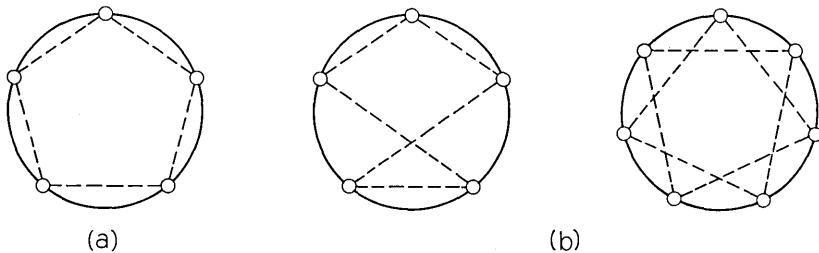
Fig. 9 — (a) Empty cycle in \tilde{G} , (b) non-cycles. Dashed edges belong to \tilde{G} ; edges not shown belong to G .
