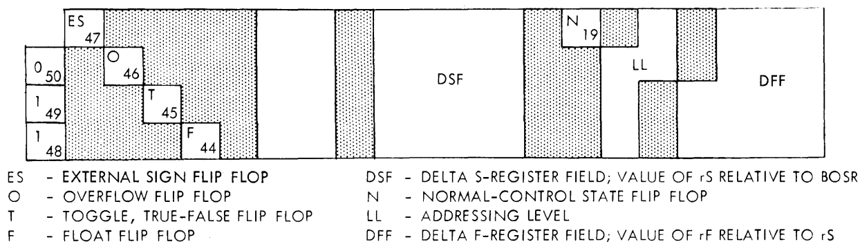
Figure 8-26. Top-of-Stack Control Word (TSCW)
