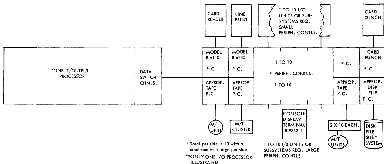
Figure 1-7. Input/Output Subsystem
