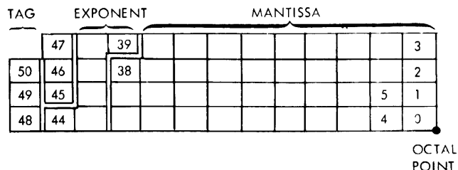
Figure 2-10. Single-Precision Operand (Hexadecimal)
