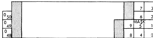
Figure 8-7. Interrupt Mask Word
