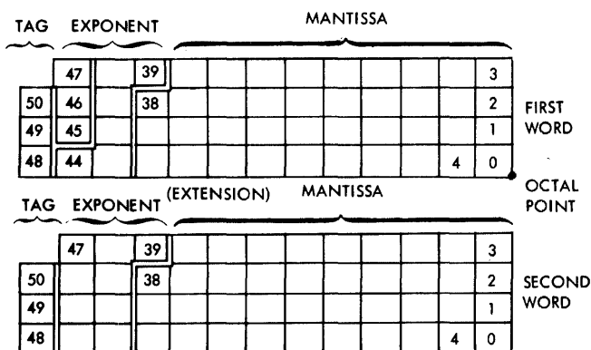
Figure 2-12. Double-Precision Operand
