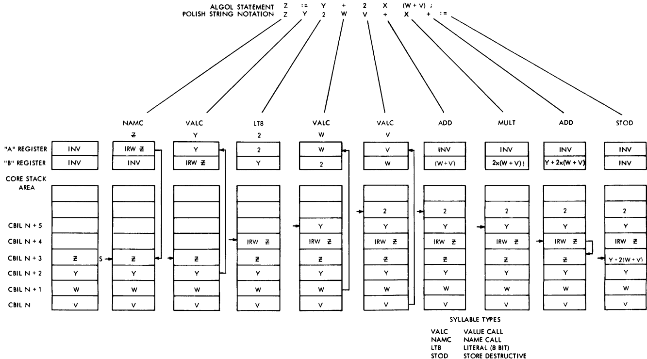
Figure 3-3. Stack Operation
