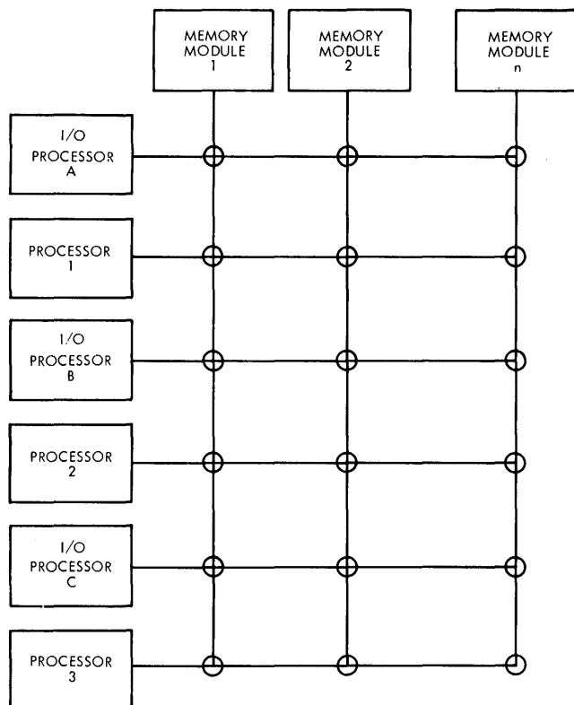
Figure 5-15. Memory Organization
