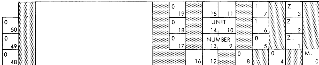
Figure 8-14. Interrogate Peripheral Unit Type Function Word
