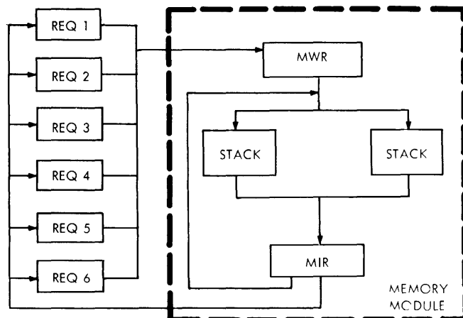
Figure 5-19. Memory Registers
