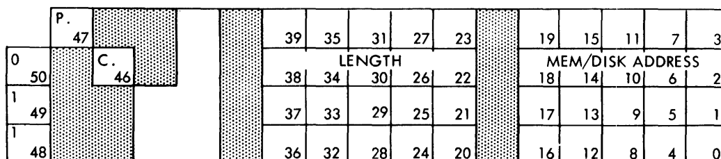
Figure 6-7. Segment Descriptor
