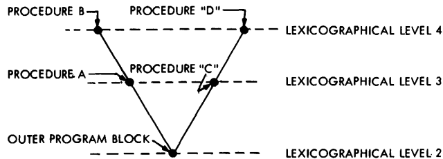
Figure 3-9. Addressing Environment Tree of ALGOL Program
