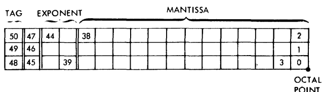
Figure 2-11. Single-Precision Operand (Octal)
