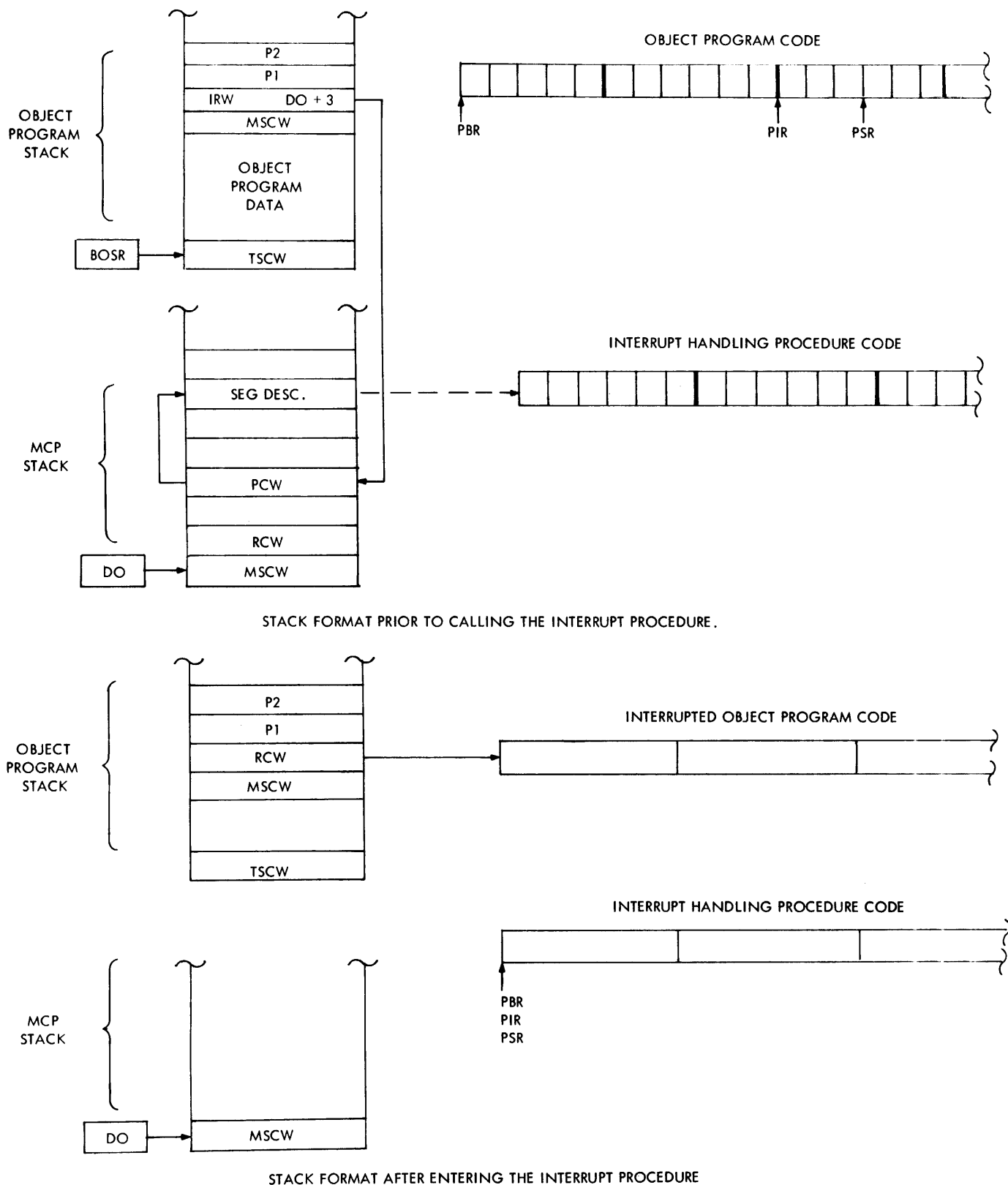
Figure 5-8. Stack Format
