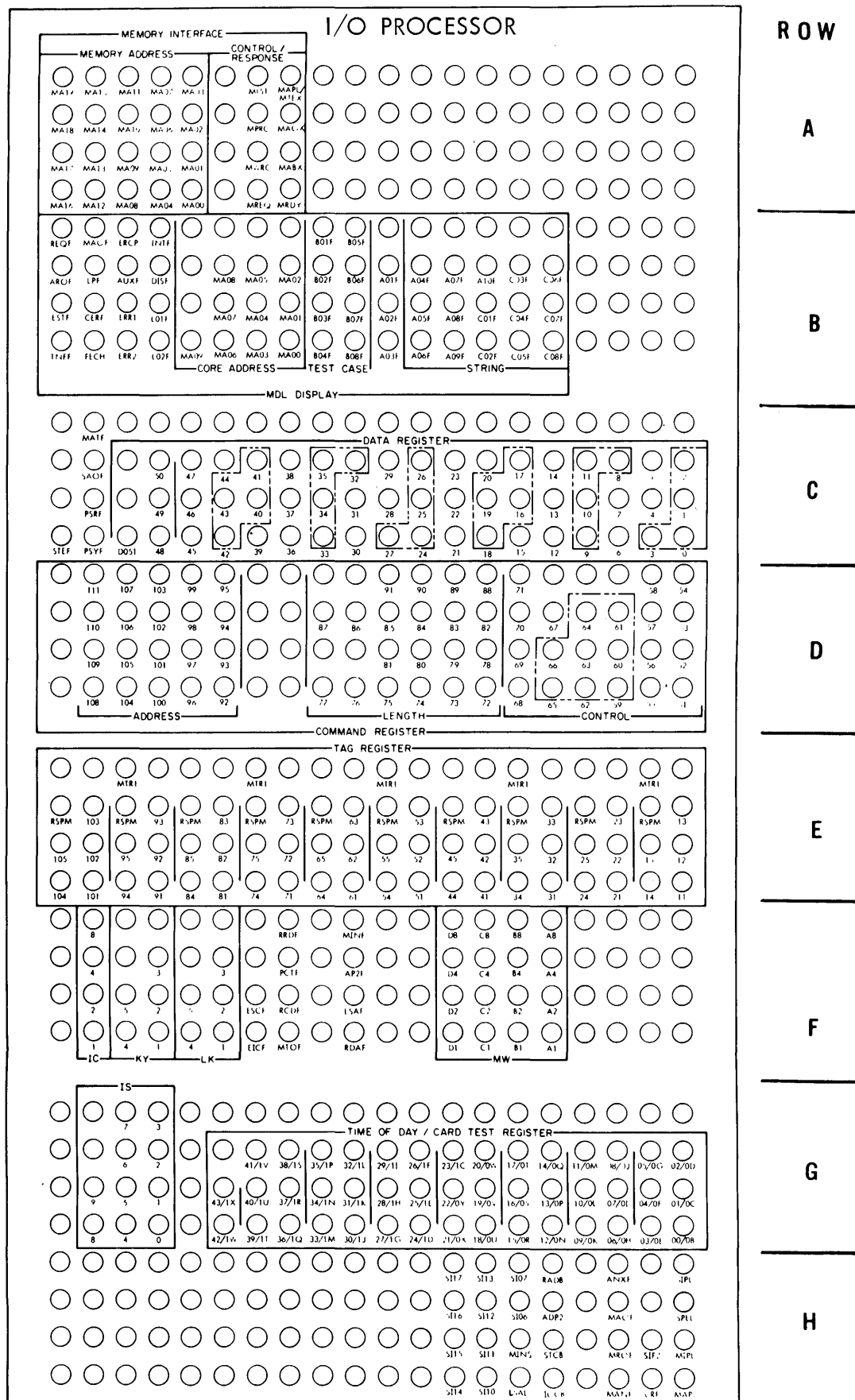
Figure 4-7. Input/Output Processor Display Panel B
