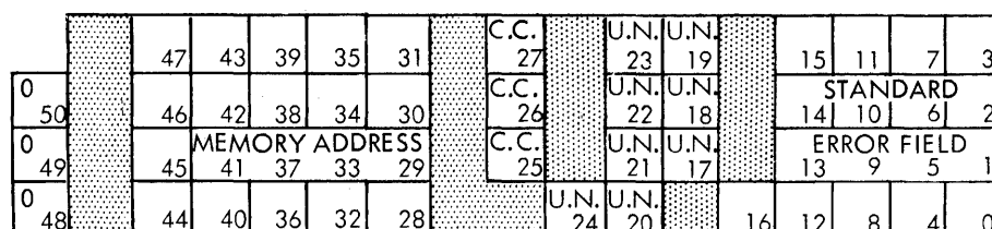
Figure 8-5. Result Descriptor
