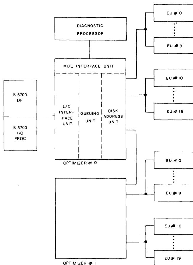
Figure 12-2. Optimizer Interfaces.
