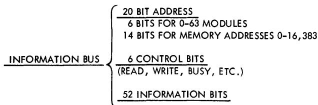
Figure 5-16. Information Transmission
