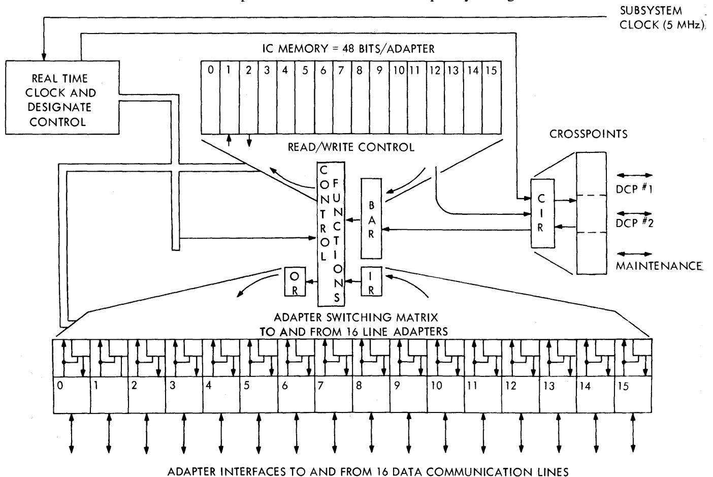
Figure 11-3. Adapter Cluster.
