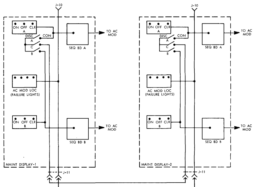
Figure 4-4. Power Control
