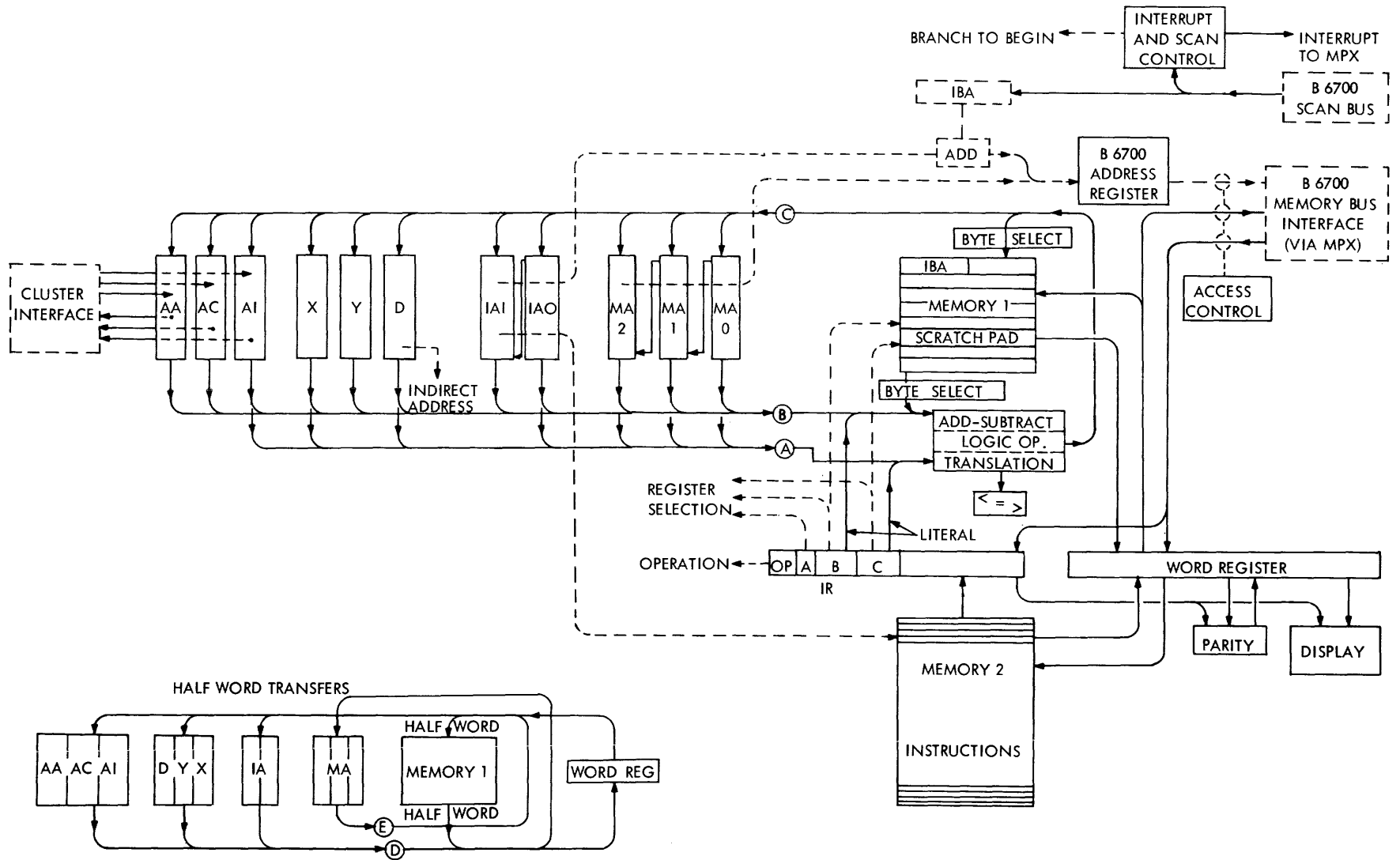
Figure 11-2. DCP Block Diagram.
