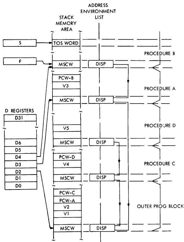
Figure 3-8. D Registers Indicating Current Addressing Environment
