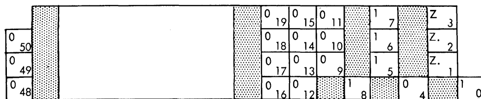
Figure 8-10. Read Interrupt Literal Function Word
