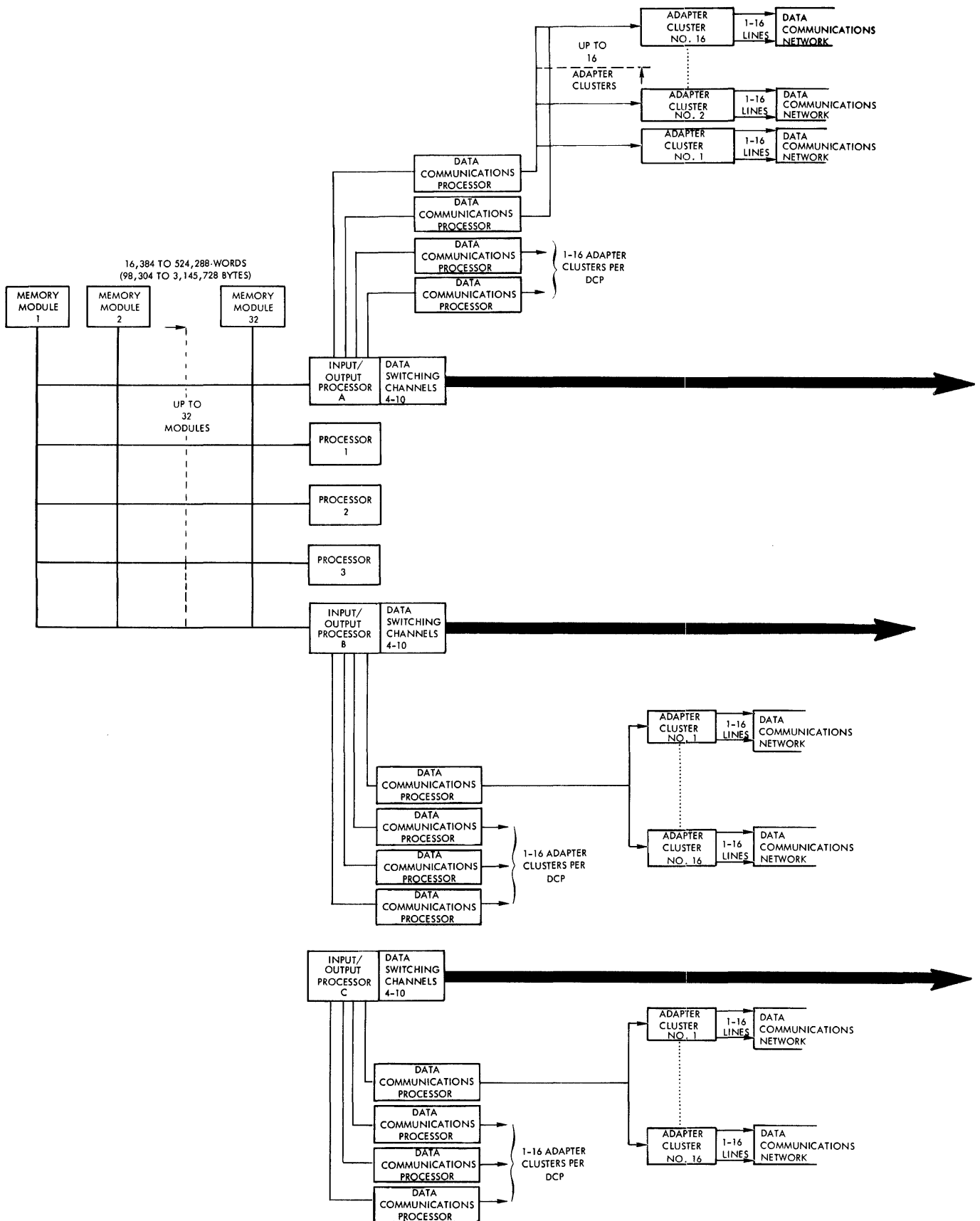
Figure 1-4. B 6700 Representative Configuration (sheet 1 of 2)
