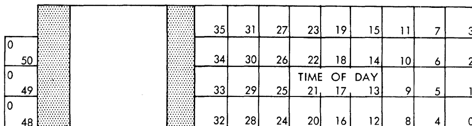
Figure 8-19. Time-of-Day Word
