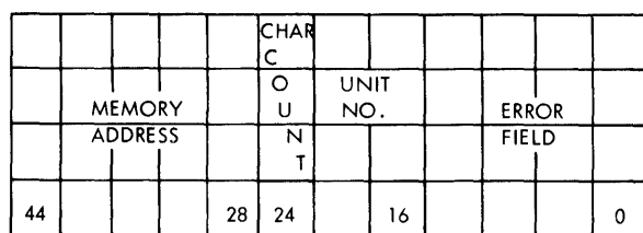
Figure 10-3. Result Descriptor Format
