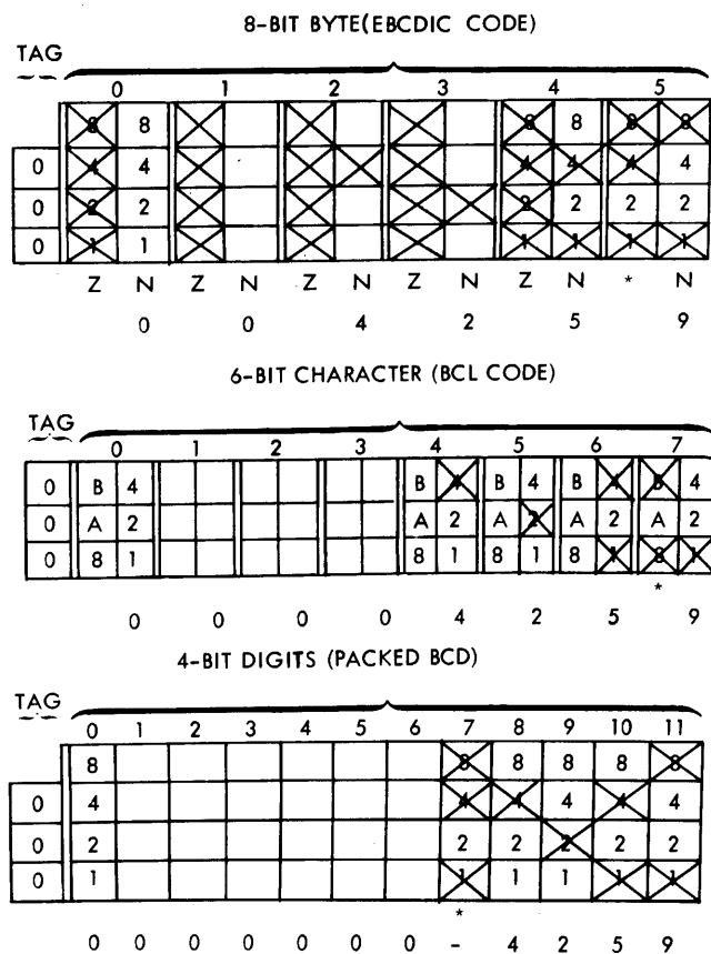
Figure 2-9. (-4259) in 8-, 6-, and 4-Bit Code
