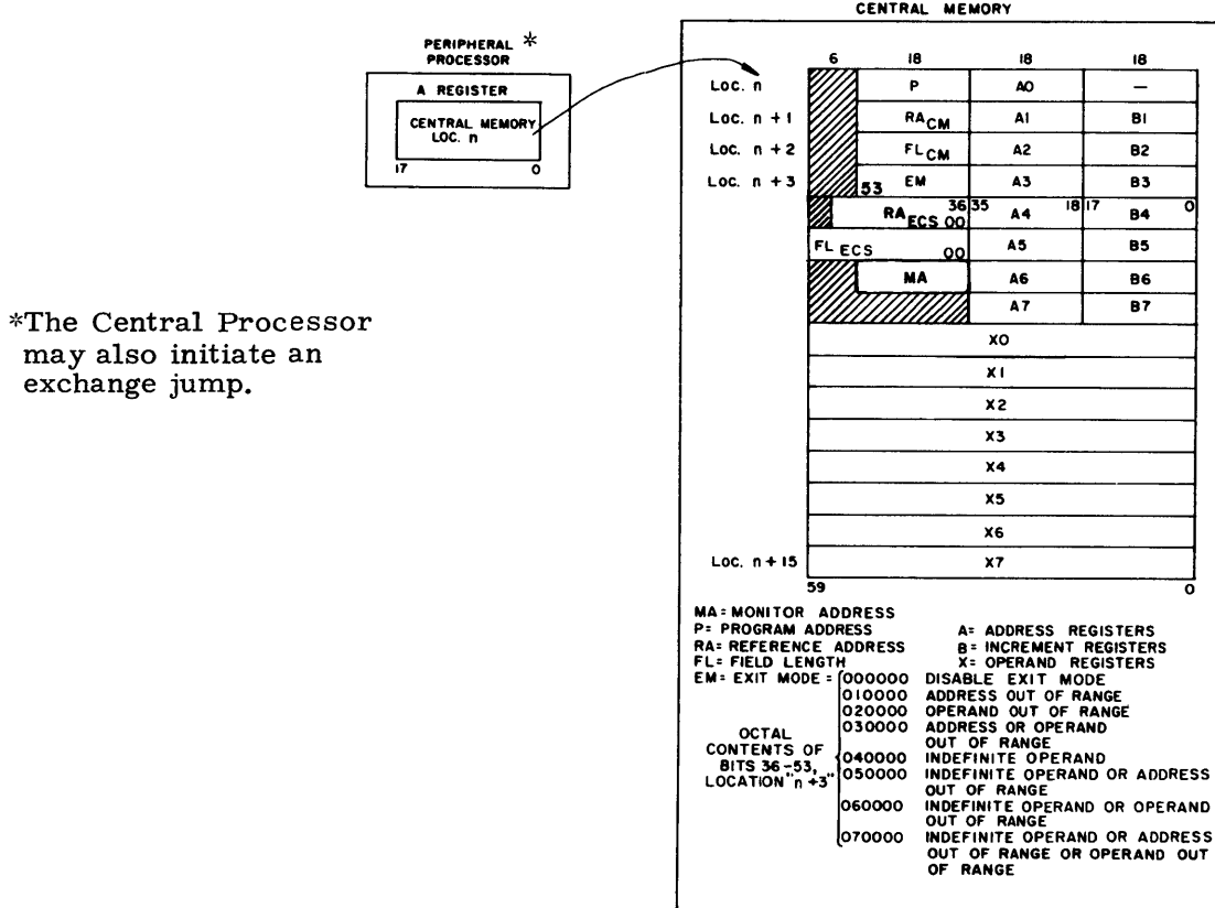
Figure 2-3. Exchange Jump Package
