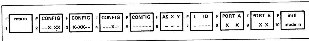
Figure B-3. Terminal Installation Parameters
