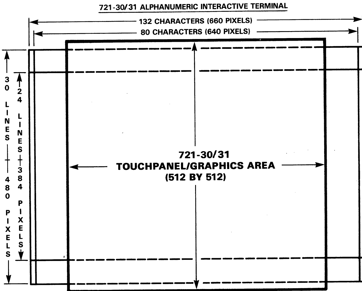
Figure 2-1. Display Screen Layout
