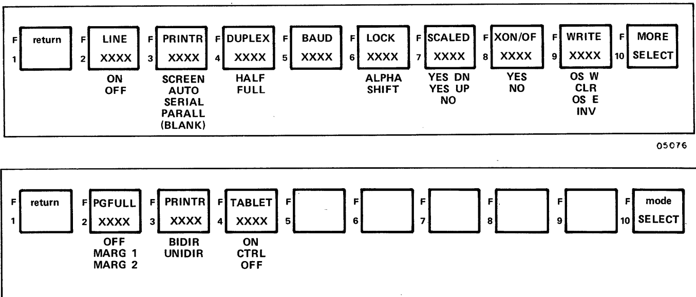
Figure 2-5. Operator Parameters Display
