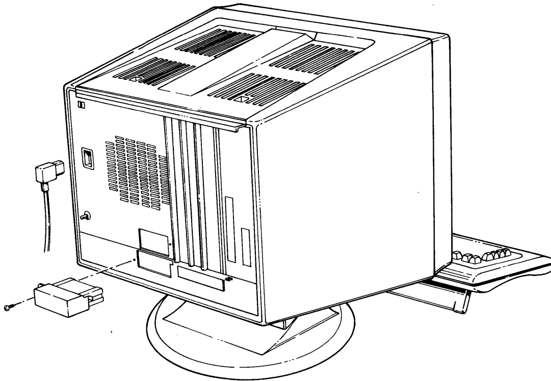
Figure B-1. Memory Module Insertion
