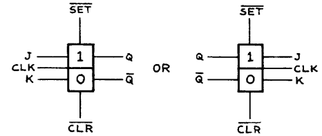
J/K FLIP-FLOP
