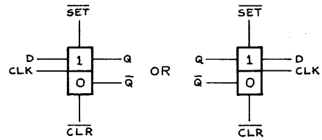
D-TYPE FLIP-FLOP
