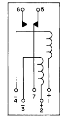
K1, K2, K3, K4 BOTTOM VIEW
