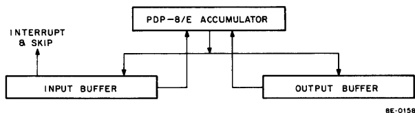
Figure 6-1 12-Channel Buffered Digital I/O -Block Diagram
