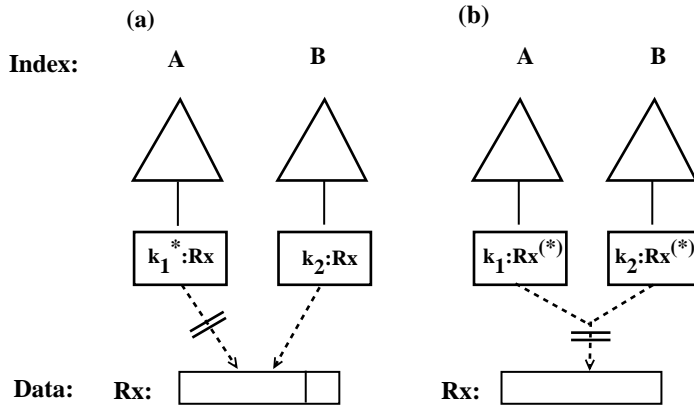
Figure 1: Locking key values is contrasted with locking records for locking ranges. (a) Locking a range and key on a path, here from index A, permits accesses through other indexes, here index B. (b) A record lock used as a range lock locks all paths that involve attributes from the record, here paths from indexes A and B. It also locks the access path that bypasses all indexes.
