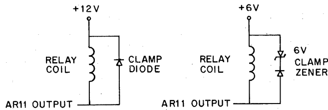
Figure 4-3 Clamping Circuits for Inductive Loads
