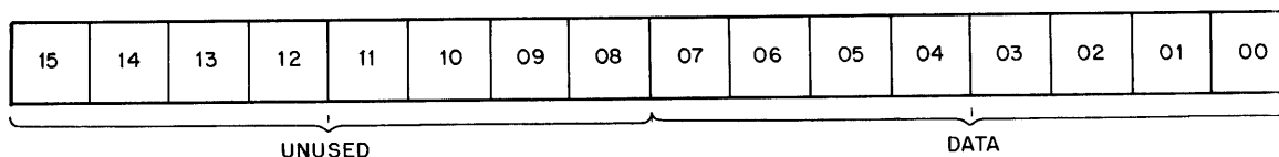
Figure 3-3 Clock Buffer/Preset Register
