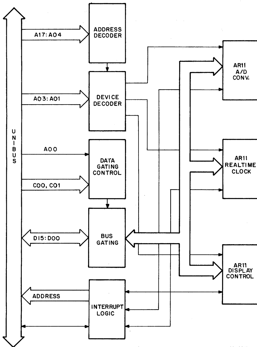
Figure 1-1 AR11 Block Diagram
