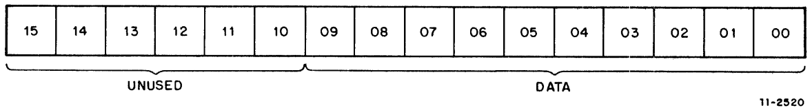
Figure 4-5 X and Y Buffer Registers
