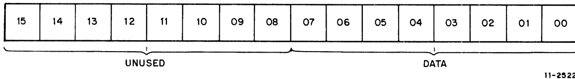
Figure 3-4 Clock Counter Register
