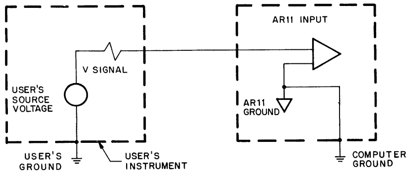
Figure 2-1 AR11 Input Referenced to User's Ground
