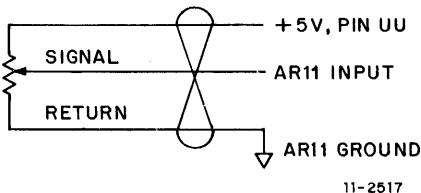
Figure 2-3 Use of +5 V Supply Output
