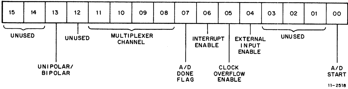
A/D Status Register
