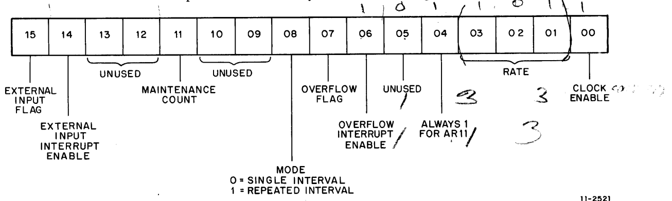
Figure 3-2 Clock Status Register
