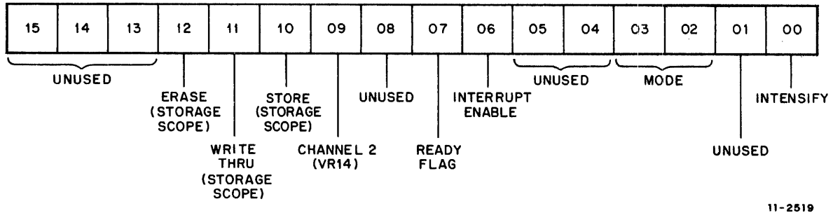
Figure 4-4 Display Status Register
