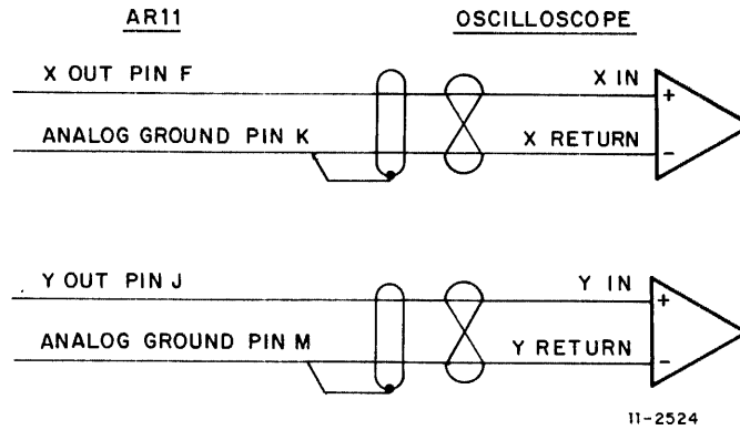
Figure 4-2 Connection to Oscilloscope with Differential Input
