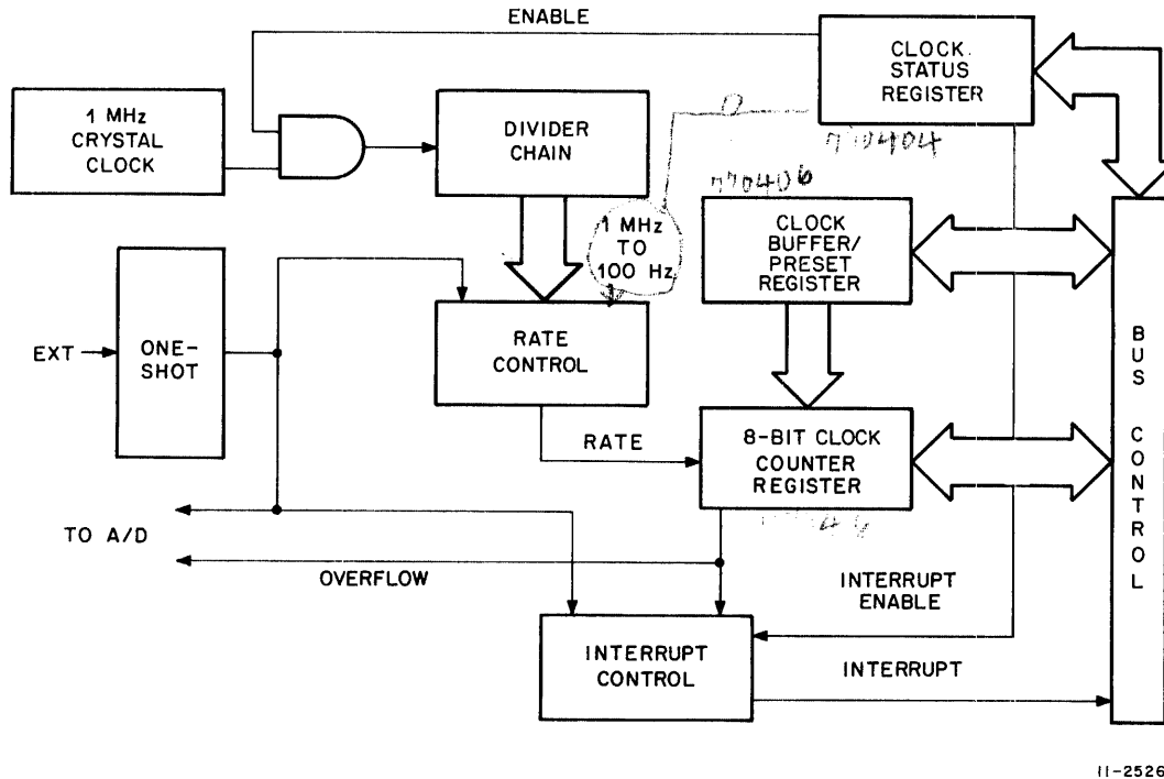
Figure 3-1 Clock Block Diagram
