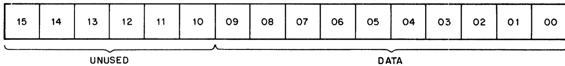
Figure 2-5 A/D Buffer Register (Read Only)
