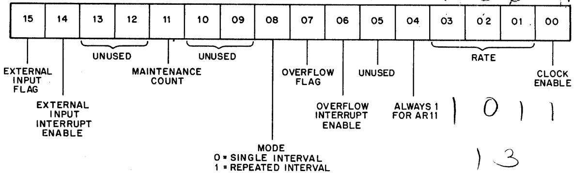
Clock Status Register
