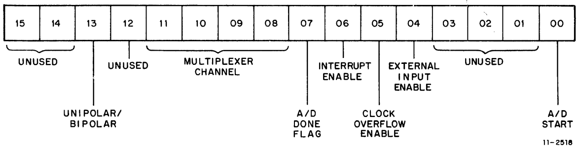
Figure 2-4 A/D Status Register
