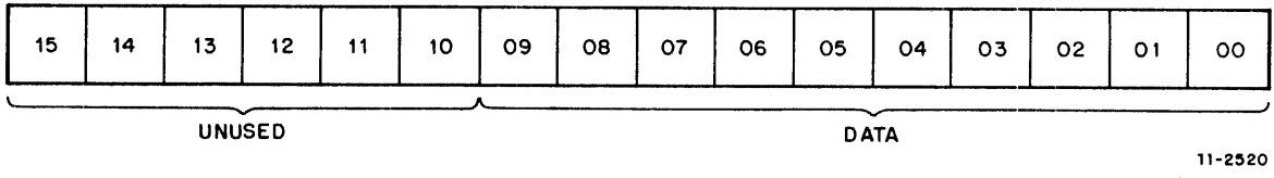
A/D Buffer Register
