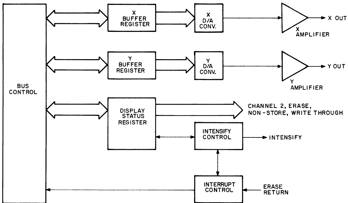
Figure 4-1 Display Control Block Diagram
