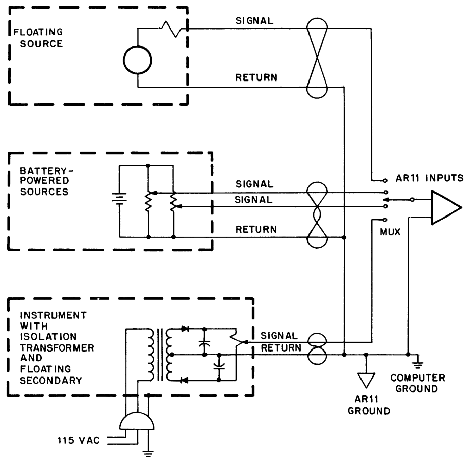
Figure 2-2 Floating AR11 Input Signals
