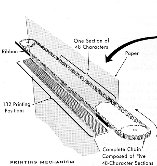
Figure 7. IBM 1403 Printer
