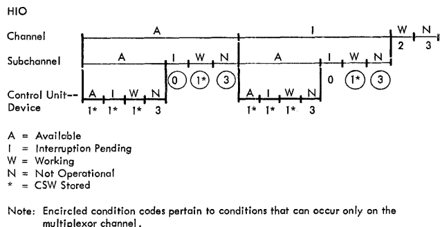
Figure 25. Condition Code set by HALT I/O
