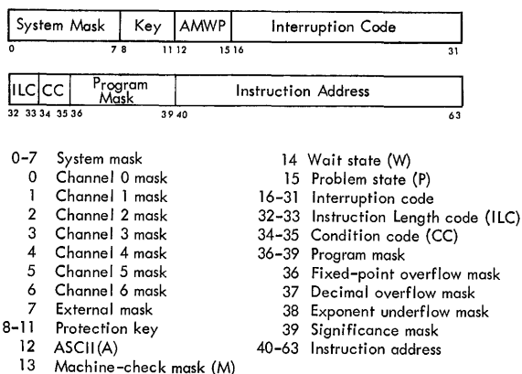
● Figure 14. Program Status Word Format
