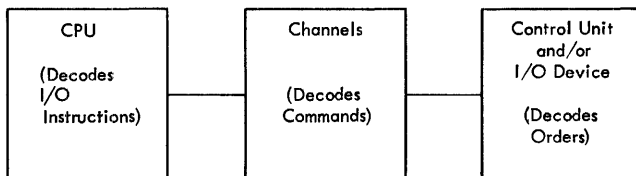
Figure 20. Relationship of I/O Instructions, Commands, and Orders
