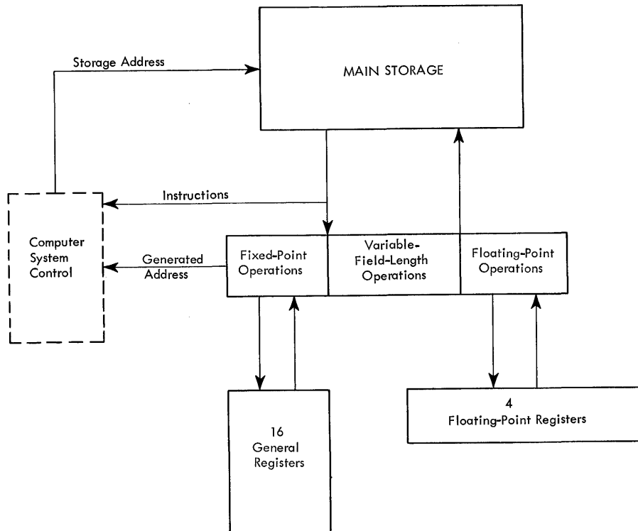
Figure 4. Basic Concept of Central Processing Unit Functions
