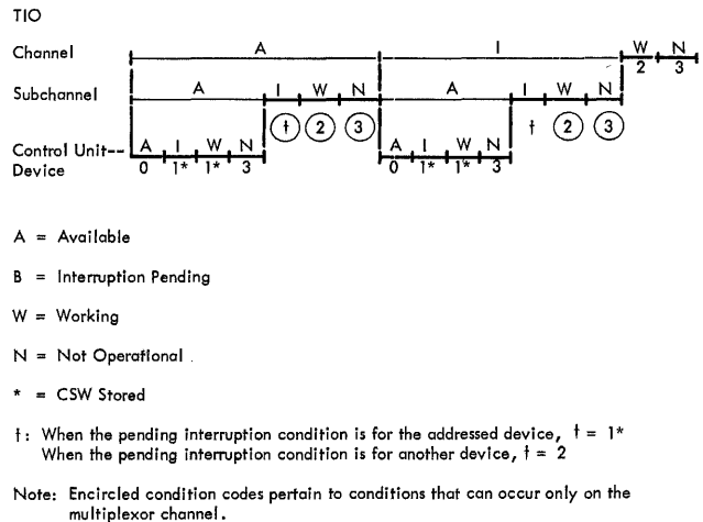
Figure 24. Condition Code set by TEST I/O
