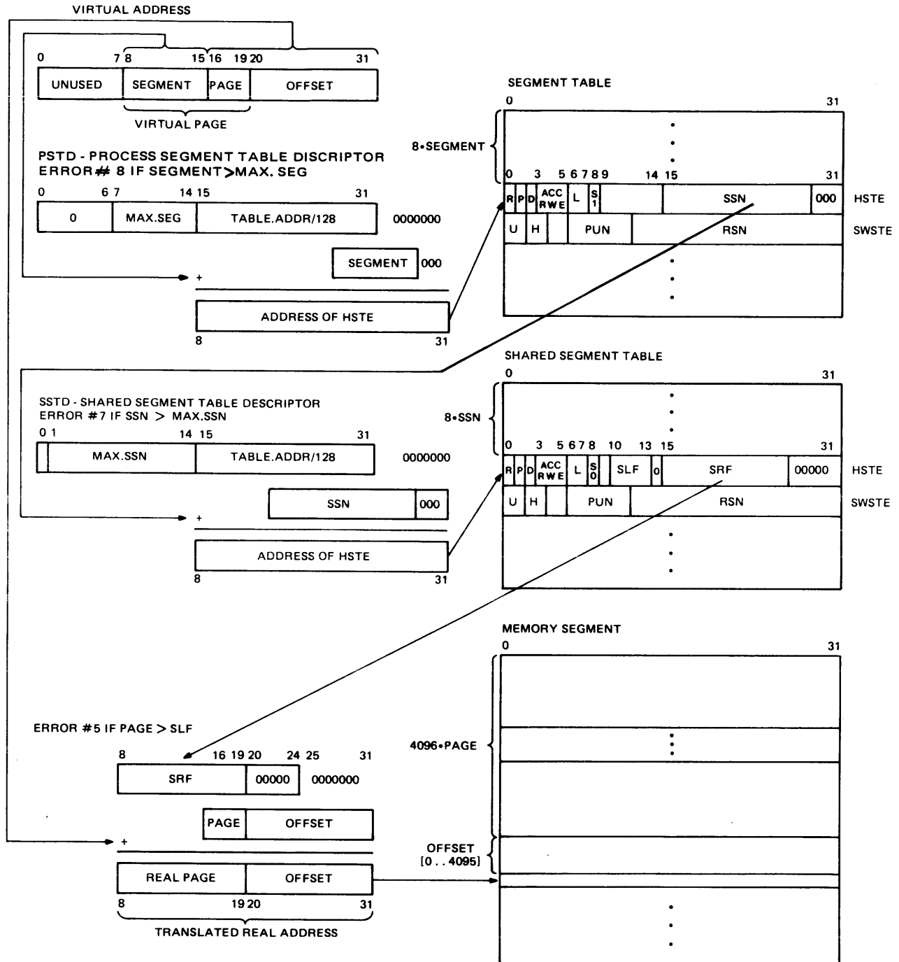
Figure 11-4 MAT Translation, Shared Segment
