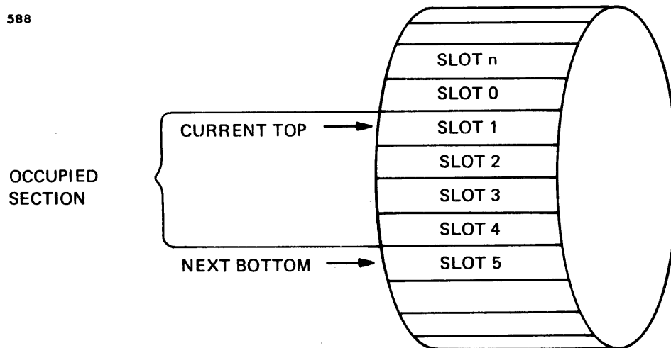
Figure 3-4 Circular List
