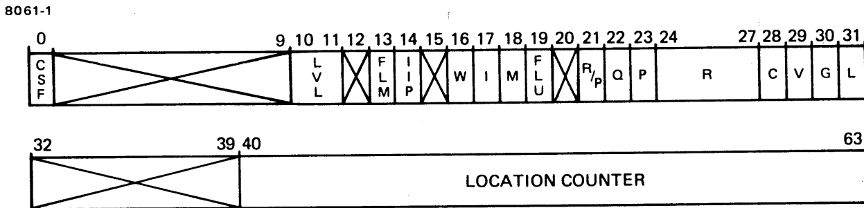
Figure 1-2 Program Status Word
