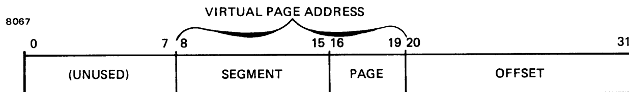
Figure 11-5 Virtual Address
