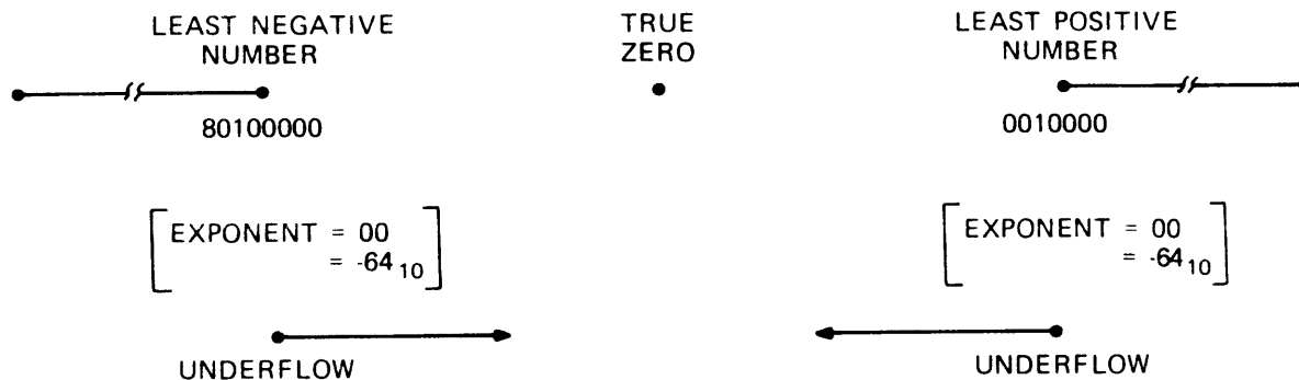
Figure 6-2 Exponent Underflow
