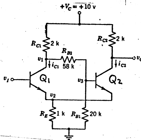
Figure 2: The Schmitt Trigger
