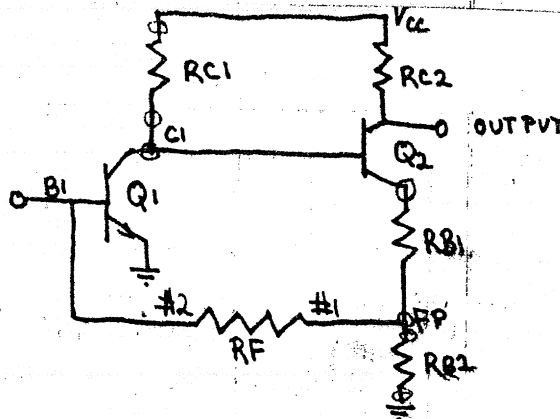
Figure 16 : Feedback Amplifier Ambiguities
