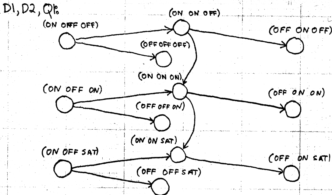
Figure 12 : State Diagram for DTL-inverter
