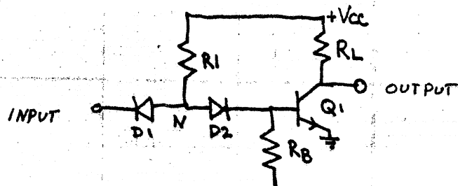
Figure 4 : DTL-Inverter
