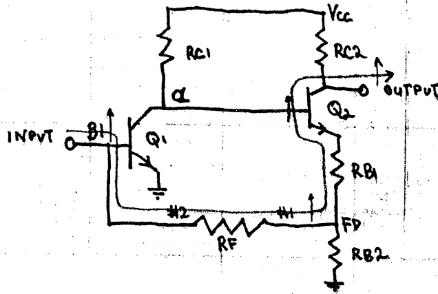
Figure 15 : Feedback Amplifier
