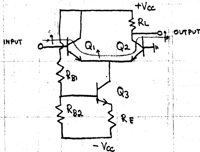
Figure II : Emitter-Coupled Pair
