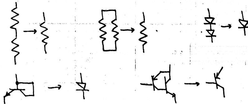
Figure 18 : Local Topological Transformations
