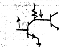
Figure 9 : Collector Current Pulling down Node Voltage
