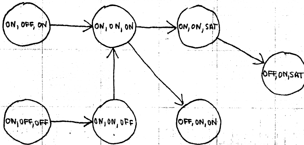
Figure 13 : State Diagram for DTL-Inverter after Simplification
