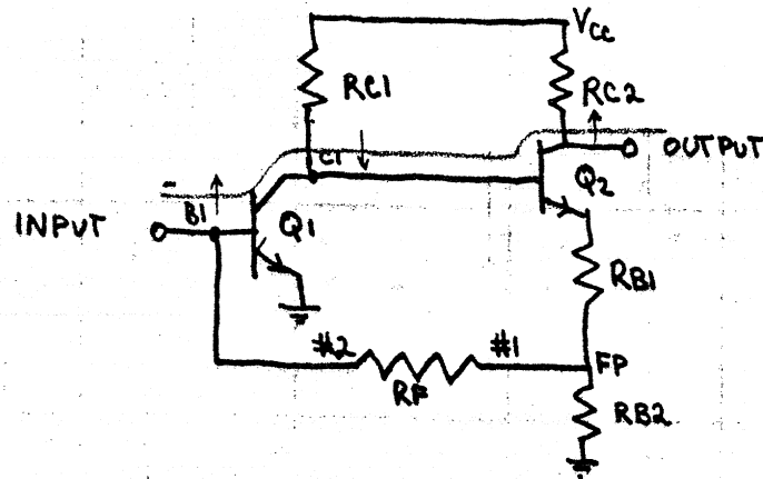
Figure 14 : Feedback Amplifier
