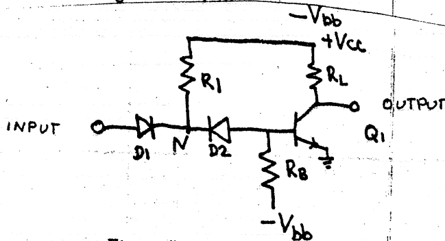
Figure 5 : Faulty DTL-Inverter
