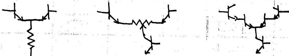
Figure 19 : Emitter-Coupled Pairs
