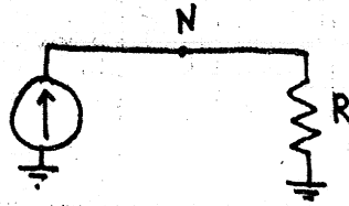
Figure 10 : KCL-Heuristic Network Assumption
