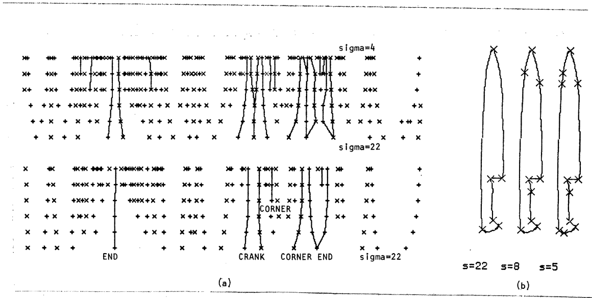
Figure 17. a. The positions of the local positive maxima (+) and negative minima (-) in the first derivatives (top) and second derivatives (bottom) for the filtered responses of the carving knife (Figure 13). Connecting lines are the part of the tree which was generated when an instance was found. b. The multiple scale interpretation of the shape.
