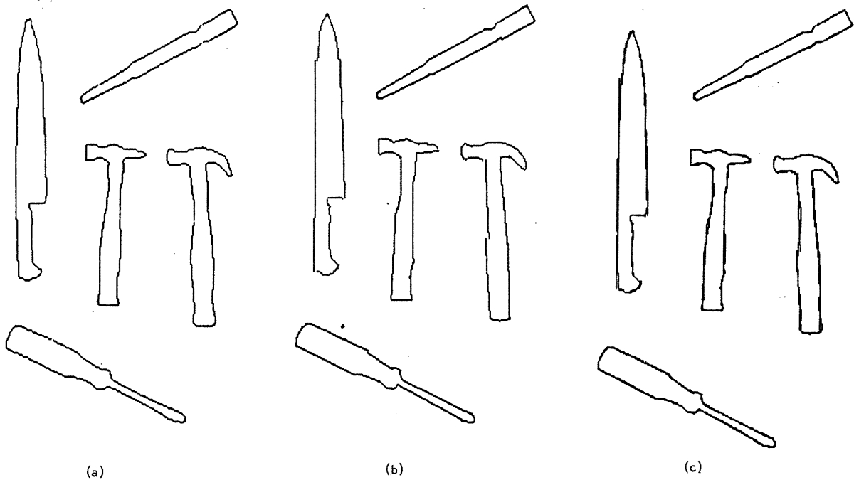
Figure 3. Illustrating the adequacy of circular splines for a set of tools. As discussed in Brady and Asada [1984], a circle may be replaced by a straight line depending on the condition number of the best fitting circle equations. a. The original contour. b. The circular spline approximation after finding the significant changes of curvature. c. Overlay of b on a.
