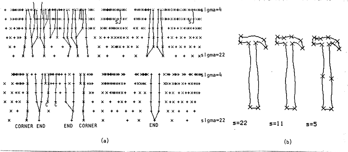
Figure 18. a. The positions of the local positive maxima (+) and negative minima (-) in the first derivatives (top) and second derivatives (bottom) for the filtered responses of the Warrington hammer (Figure 14). Connecting lines are the part of the tree which was generated when an instance was found. b. The multiple scale interpretation of the shape.
