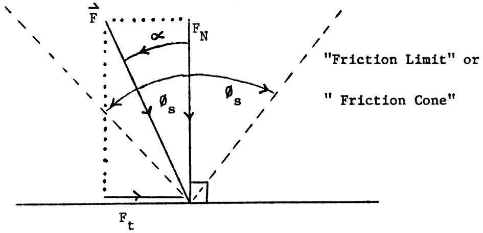
Figure 1. Friction Principles
