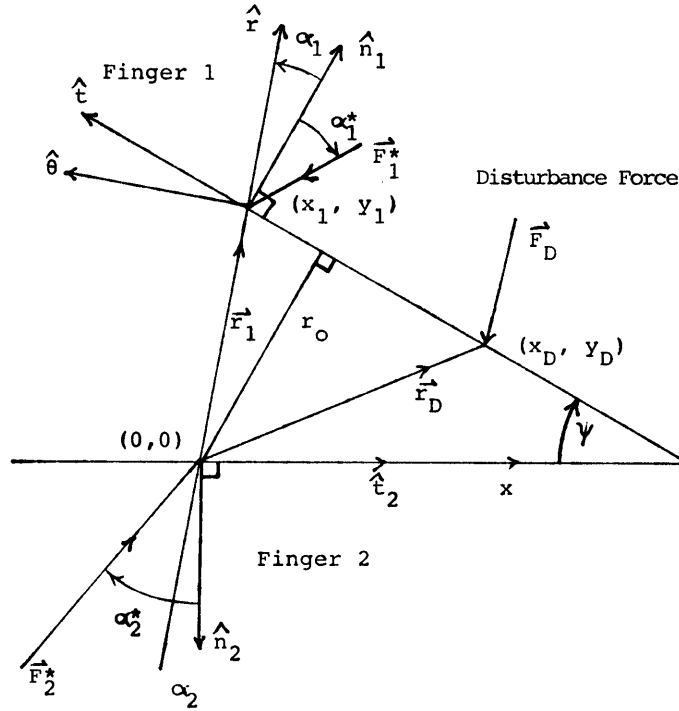
Figure 10. Grasping with Disturbance Forces
