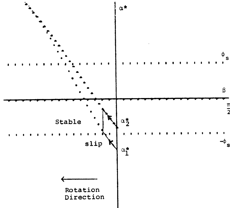
Figure 12. Rotation Due to Gravity
