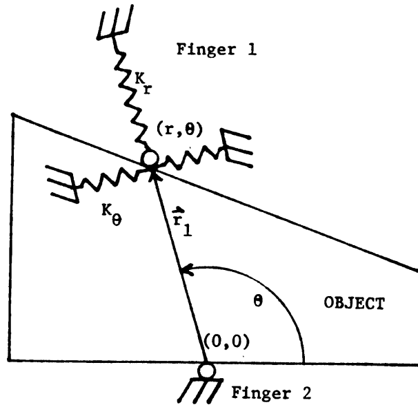
Figure 6. Polar Stiffness Representation
