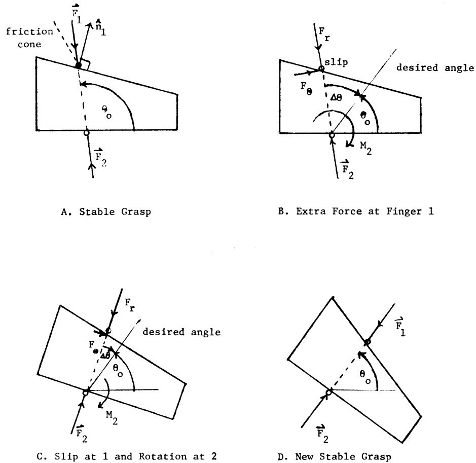
Figure 15. Part Rolling
