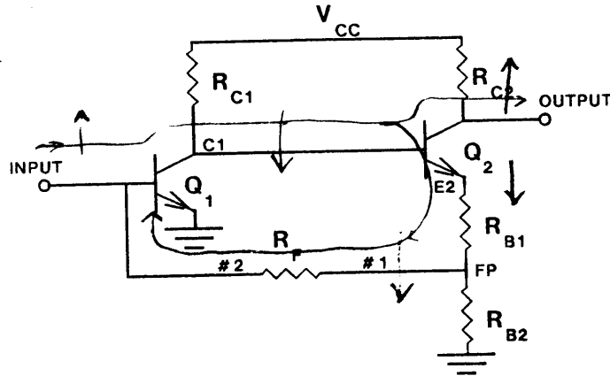
Figure 6 : CE-FEEDBACK
