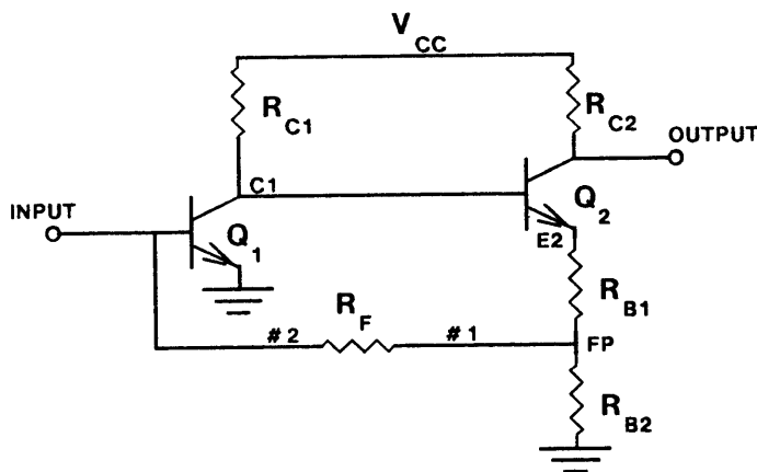
Figure 4 : CE-FEEDBACK
