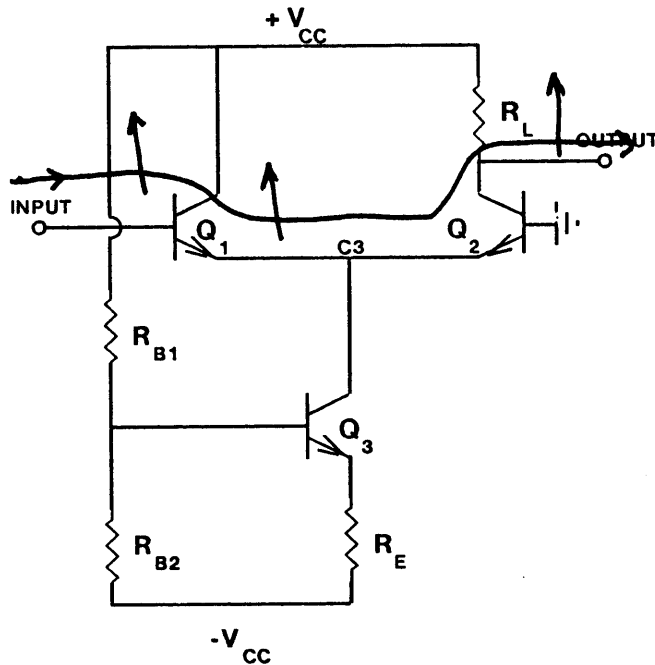
Figure 10 : Emitter-Coupled Pair
