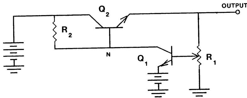
Figure 2 : Simple Power Supply
