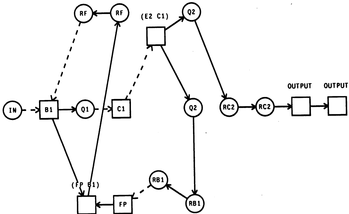
Figure 5 : Mechanism Graph for Correct Interpretation
