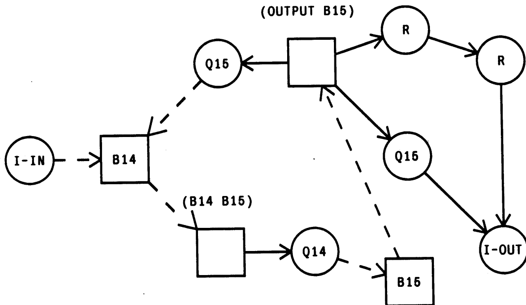
Figure 17 : Mechanism Graph for Current Limiter
