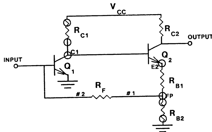
Figure 3 : Feedback Amplifier Ambiguities
