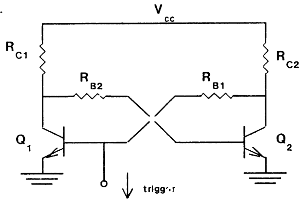
Figure 23 : Bistable Circuit
