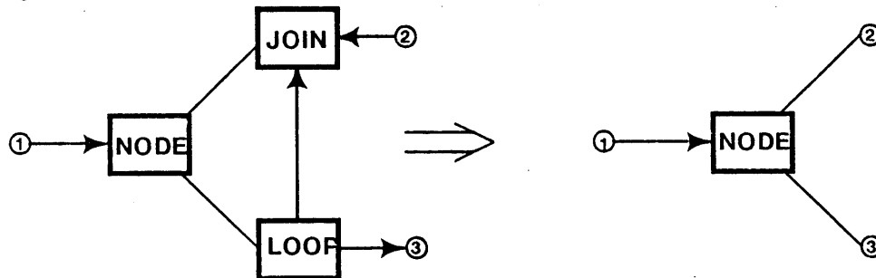
Figure 14 : Local Feedback Substitution Rule
