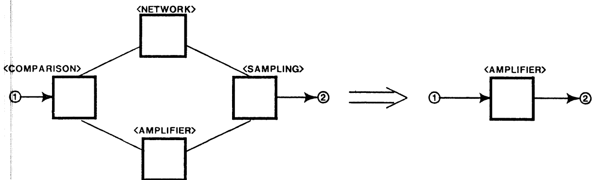
Figure 18 : General Feedback Loop
