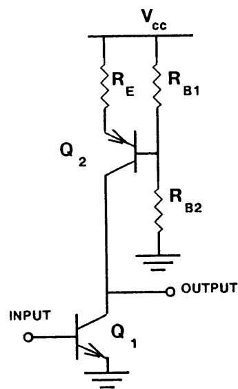
Figure 1 : Common-Emitter Amplifier with Active Load
