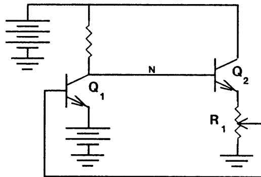
Figure 13 : Simple Power Supply as Simple Amplifier
