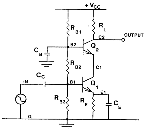
Figure 12 : A Cascode Amplifier
