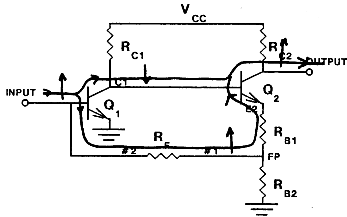
Figure 28 : Feedback as Feedforward
