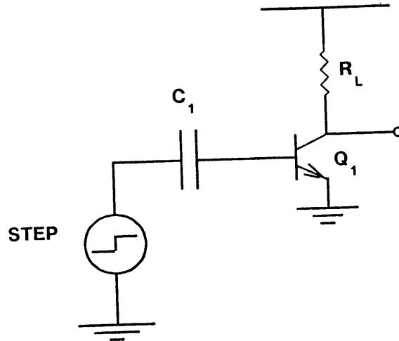
Figure 14 : Capacitor Coupling
