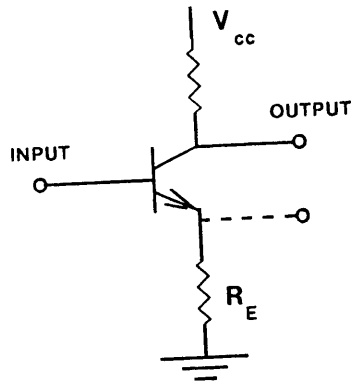
Figure 13 : Common-Emitter Amplifier
