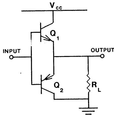
Figure 9 : Unbiased Complementary Pair
