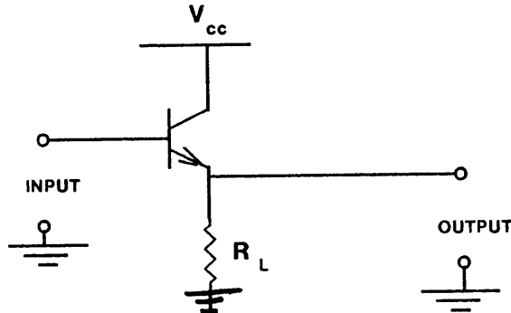
Figure 4 : Common-Collector Configuration
