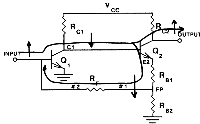
Figure 3 : Feedback Amplifier
