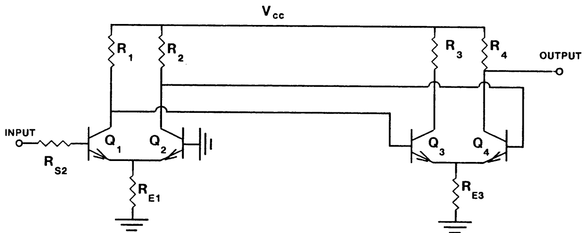
Figure 7 : Differential Amplifier Cascade
