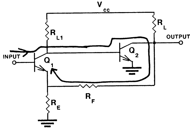
Figure 11 : Loop-Node Feedback Amplifier
