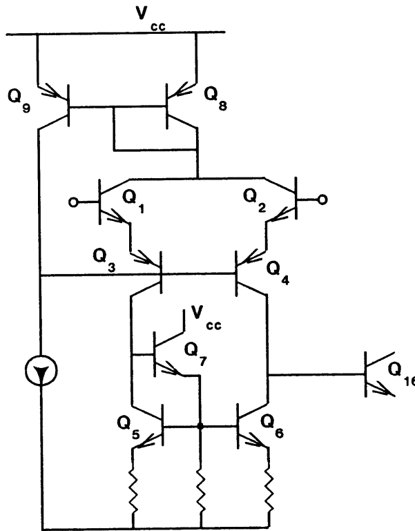
Figure 3 : 741 Input Stage
