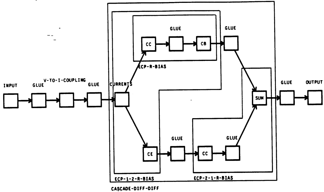
Figure 10 : Parse of Circuit of Figure 7
