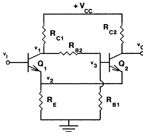
Figure 8 : Schmitt Trigger
