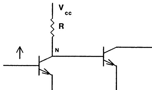
Figure 15 : KCL-heuristic Local Feedback
