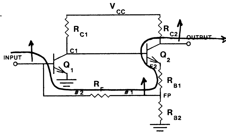
Figure 2 : Feedback Amplifier
