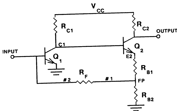
Figure 5 : Feedback Amplifier
