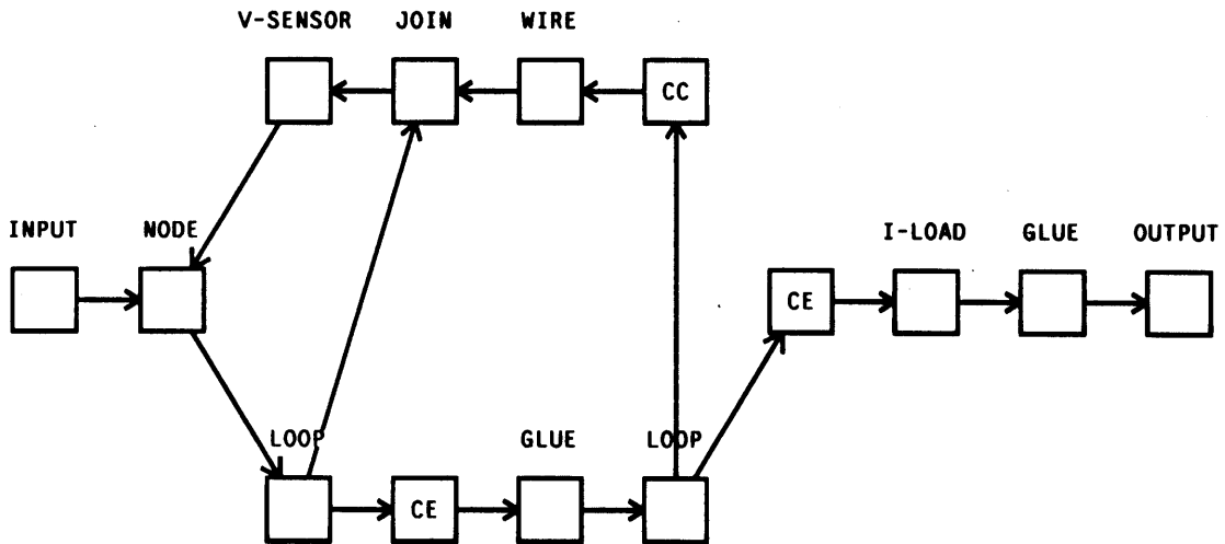
Figure 9 : Primitive Fragments of CE-FEEDBACK
