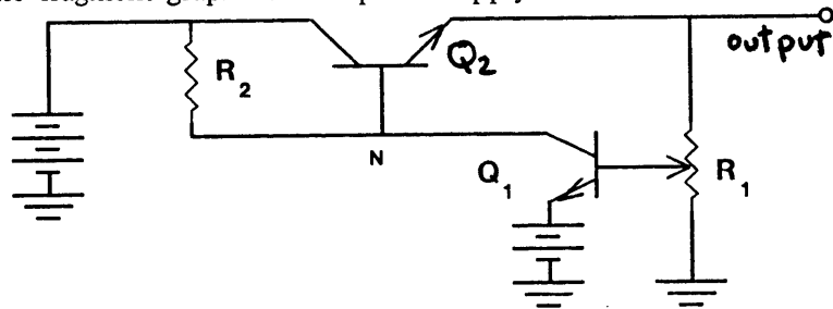
Figure 11 : Simple Power Supply
