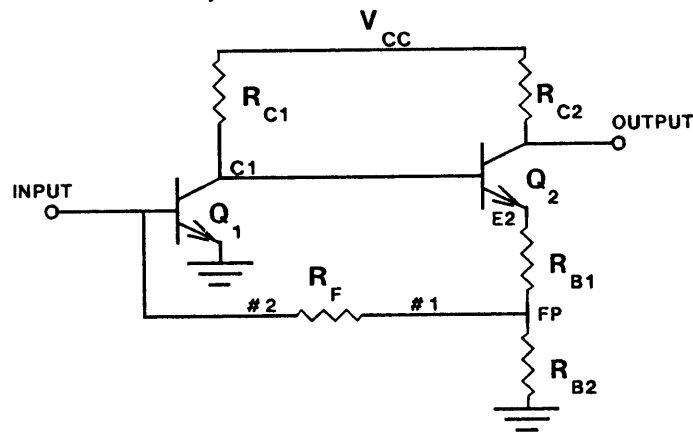
Figure 1 : Schematic for CE-FEEDBACK
