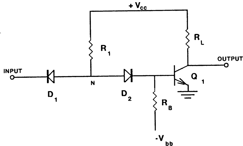
Figure 7 : DTL-inverter
