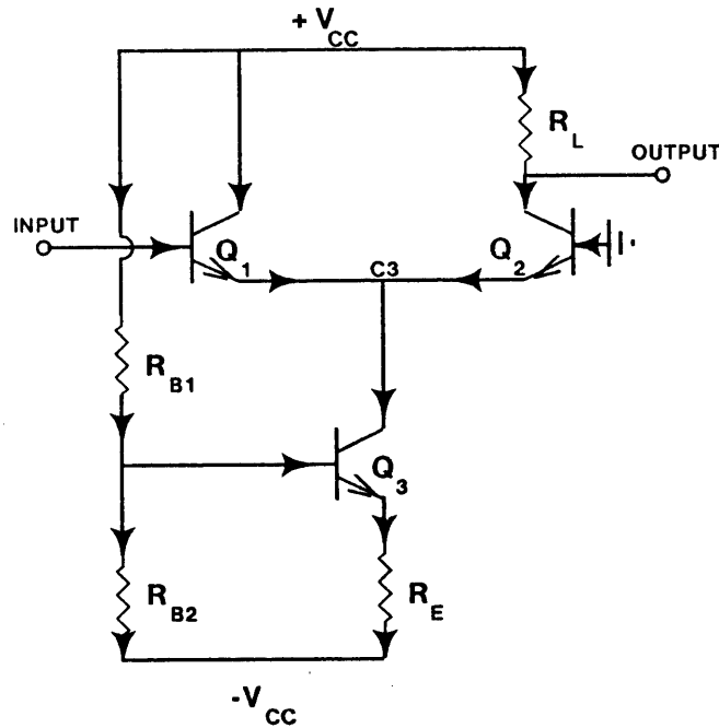
Figure 11 : Emitter-Coupled Pair
