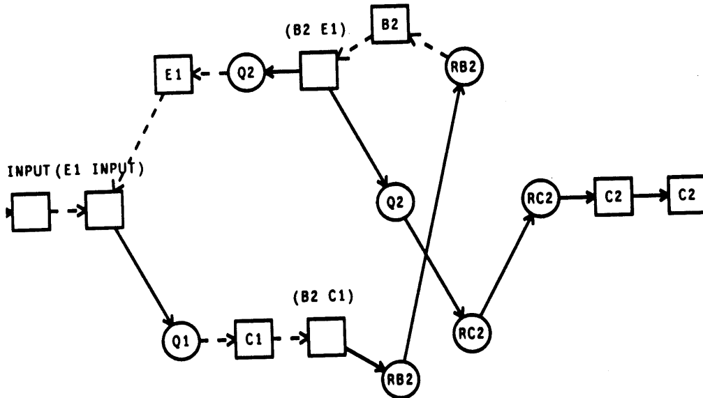
Figure 1 : Mechanism Graph of Schmitt Trigger
