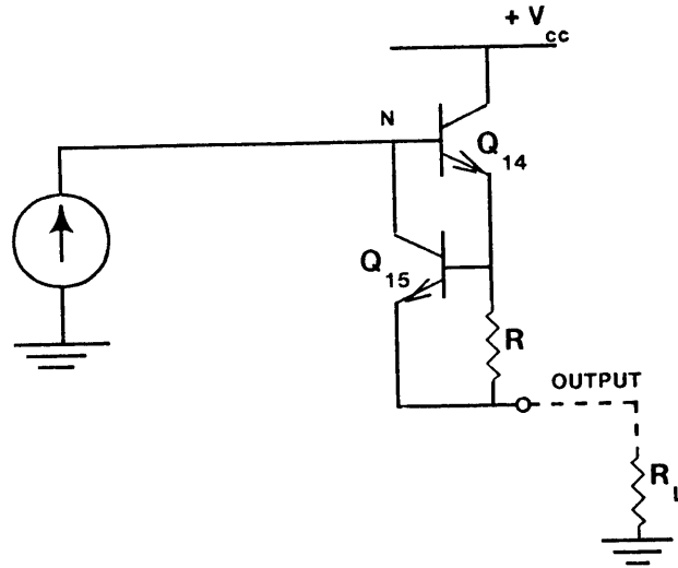
Figure 16 : Current Limiter
