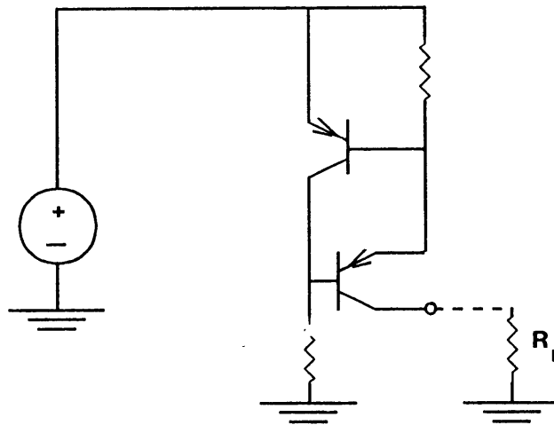
Figure 18 : Constant Current Source
