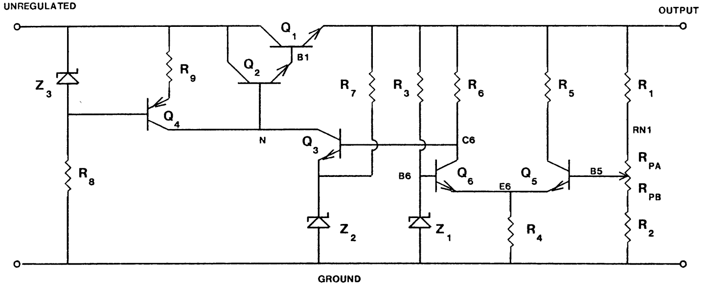
Figure 4 : Complex Power Supply
