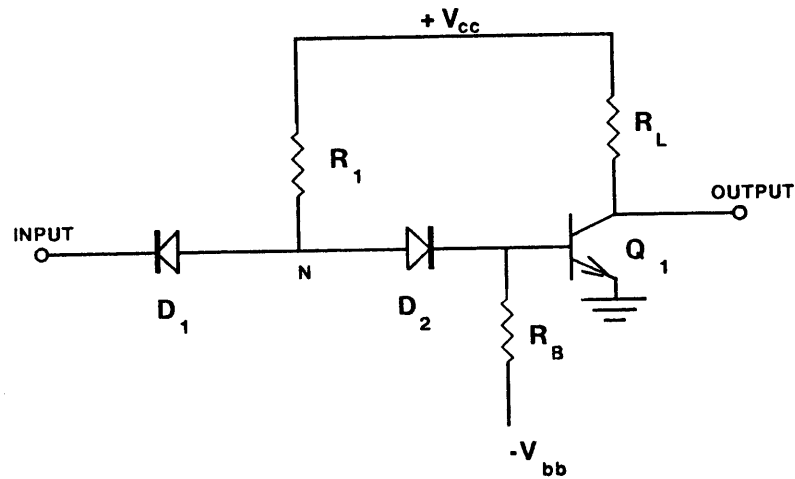
Figure 3 : DTL-Inverter
