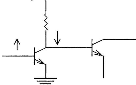
Figure 8 : Collector Current Pulling down Node Voltage
