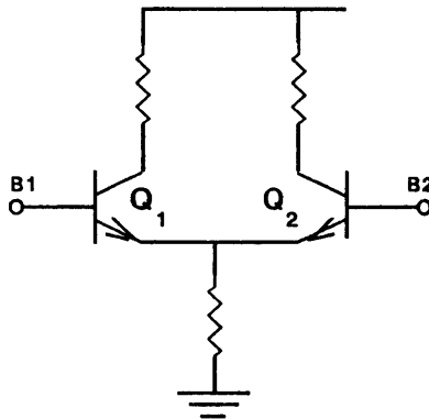
Figure 1 : Emitter-Coupled Pair
