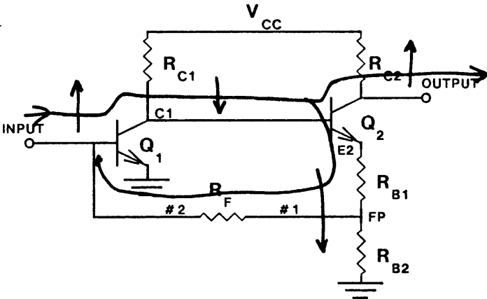
Figure 10 : Feedback Amplifier
