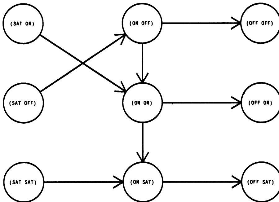
Figure 24 : Transition Diagram for Bistable Circuit
