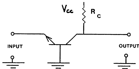
Figure 3 : Common-Base Configuration
