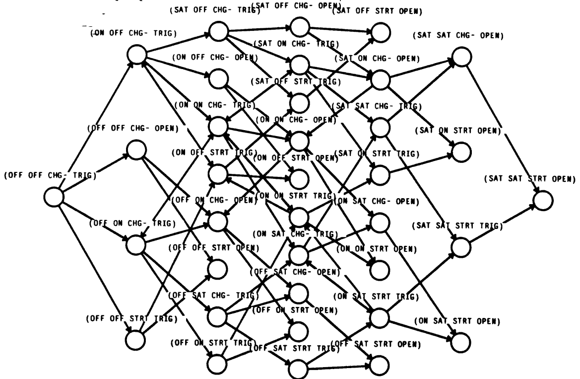
Figure 26 : State Transition Diagram For Monostable
