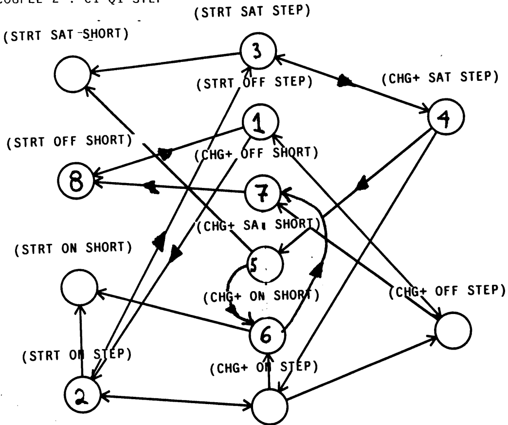
Figure 15 : State Diagram for Capacitive Coupling
