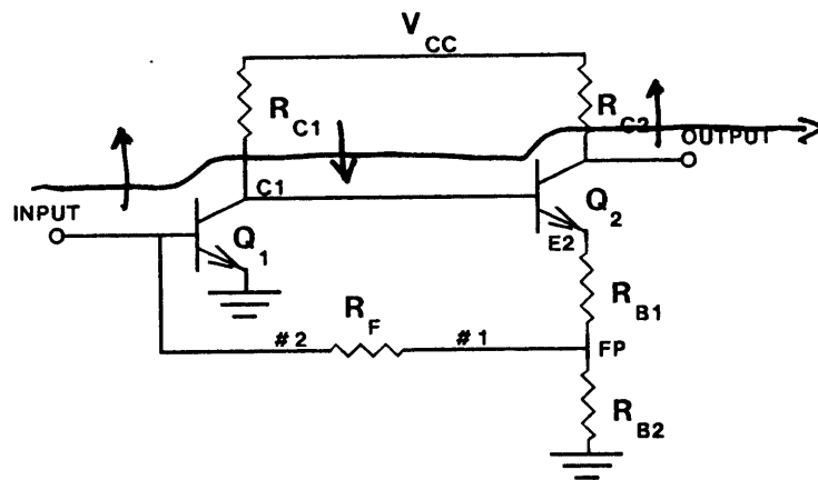
Figure 1 : Feedback Amplifier
