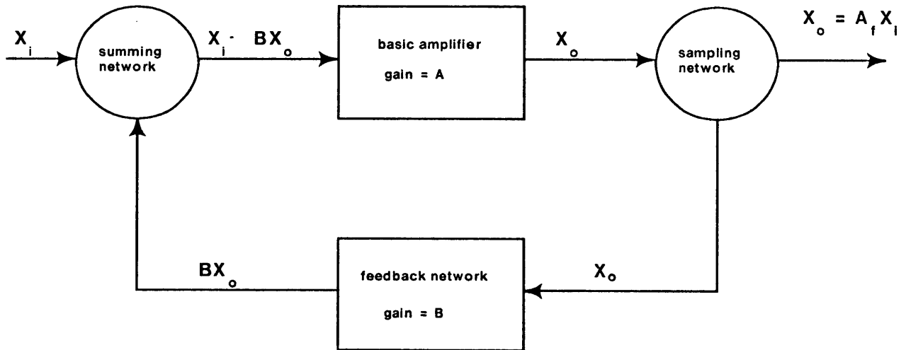
Figure 6 : Block Diagram of Feedback System
