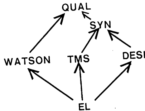
Figure 5 : Evolution of EPSP
