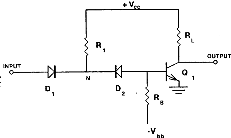
Figure 4 : Faulty DTL-Inverter
