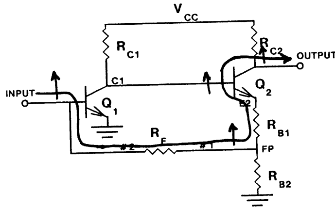
Figure 31 : CE-FEEDBACK
