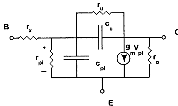
Figure 22 : Complete Hybrid- \pi Model
