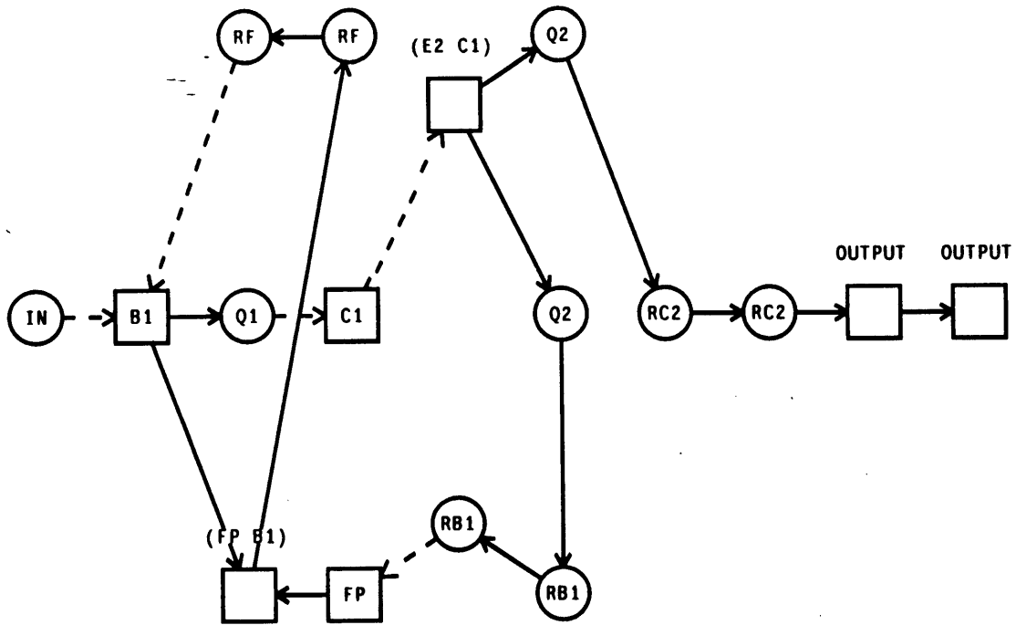
Figure 4 : Feedback Graph for Feedback Amplifier
