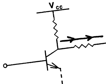
Figure 6 : Example of the V-TO-I-COUPLE Configuration
