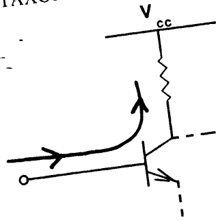
Figure 5 : Example of the I-LOAD Configuration
