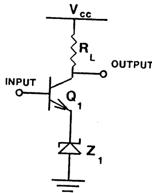
Figure 3 : Zener Bias
