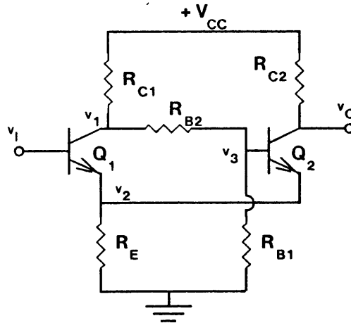
Figure 1 : The Schmitt Trigger
