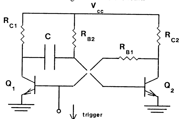
Figure 25 : Monostable Circuit
