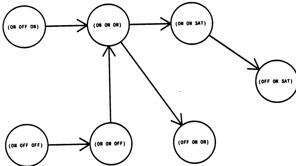
Figure 13 : State Diagram for DTL-Inverter after Simplification
