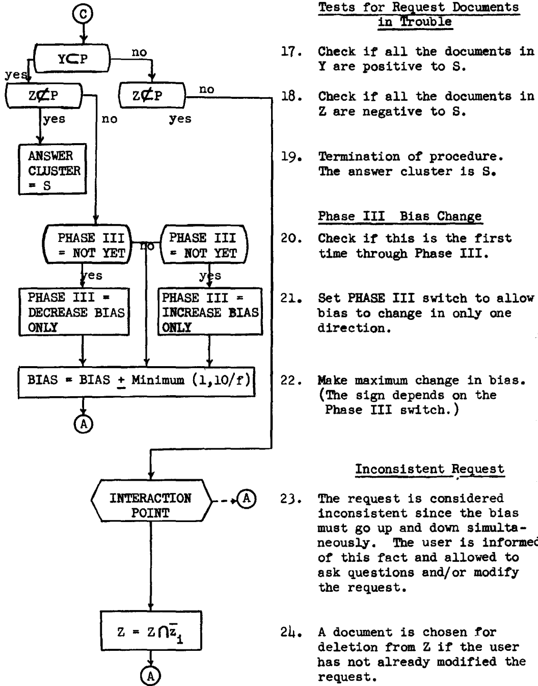
Fig. 5.6. Phase III and other tests.
