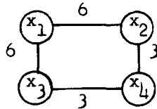
Fig. 4.5. Network containing no subset clusters.
