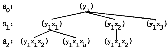
Fig. 5.11. Possible additions to S .
