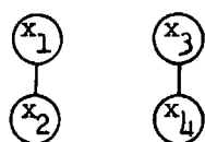
Fig. 4.4. Cluster containing unrelated subsets.
