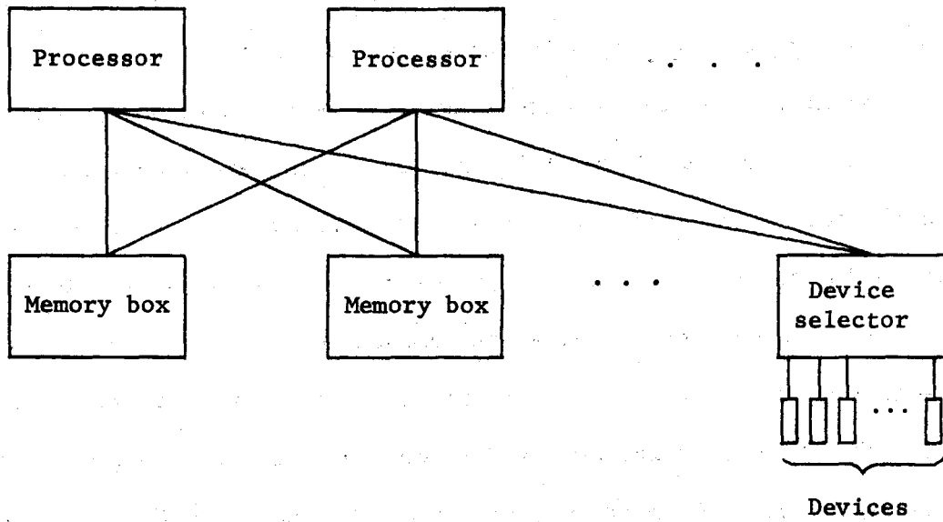
Figure 2-1: Module interconnections with devices represented as memory.
