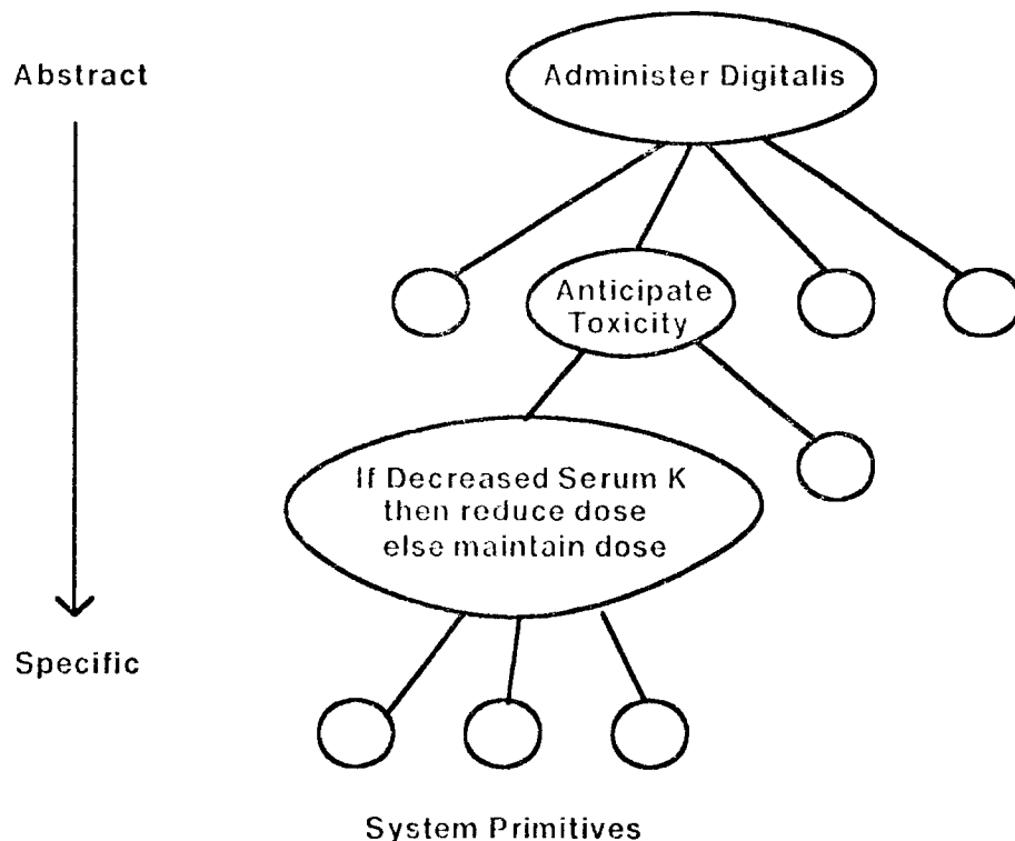
Fig. 6. Refinement Structure
