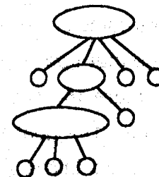
Refinement Structure
