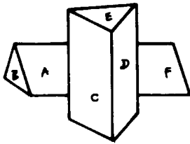
Fig. 'WEDGES'. A scene. The regions A and F have to be fused together and the result to match a region-model with shape 'parallelogram'.
