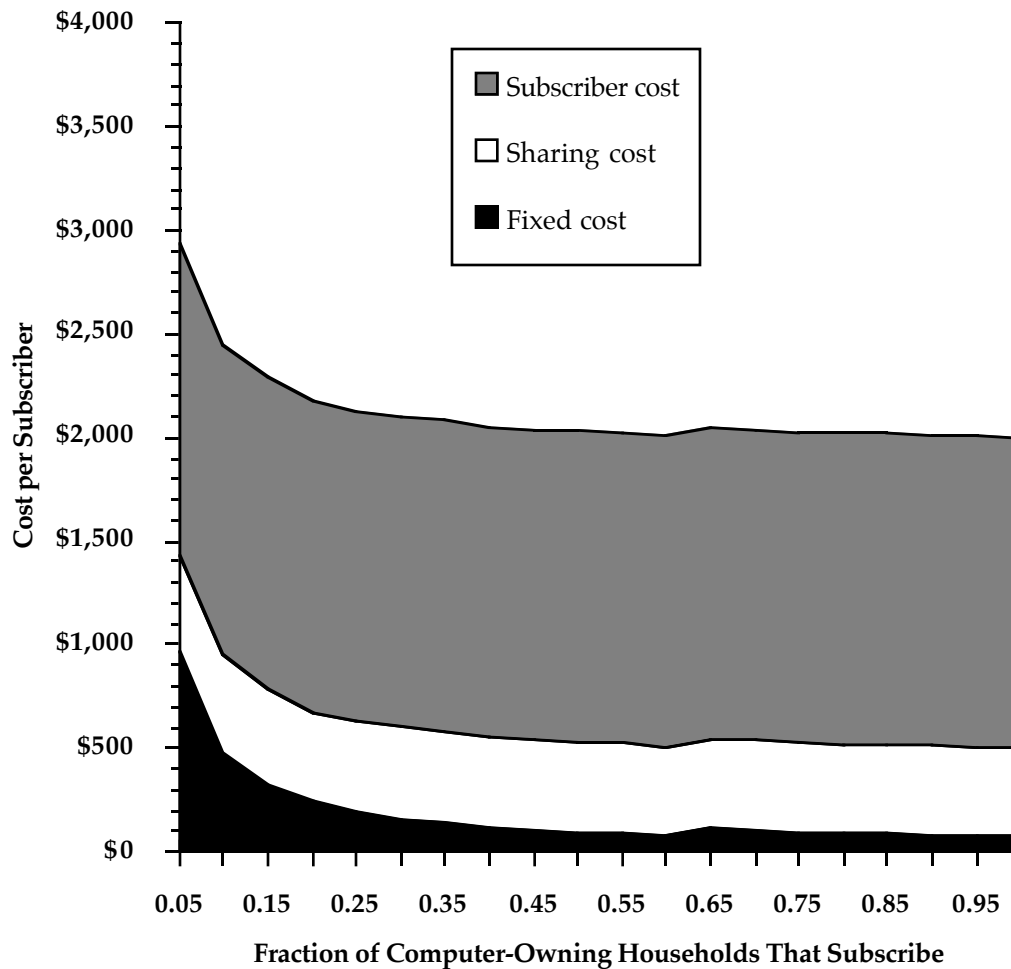
Figure 7.7: Components of average cost, 128 Kbps ISDN
