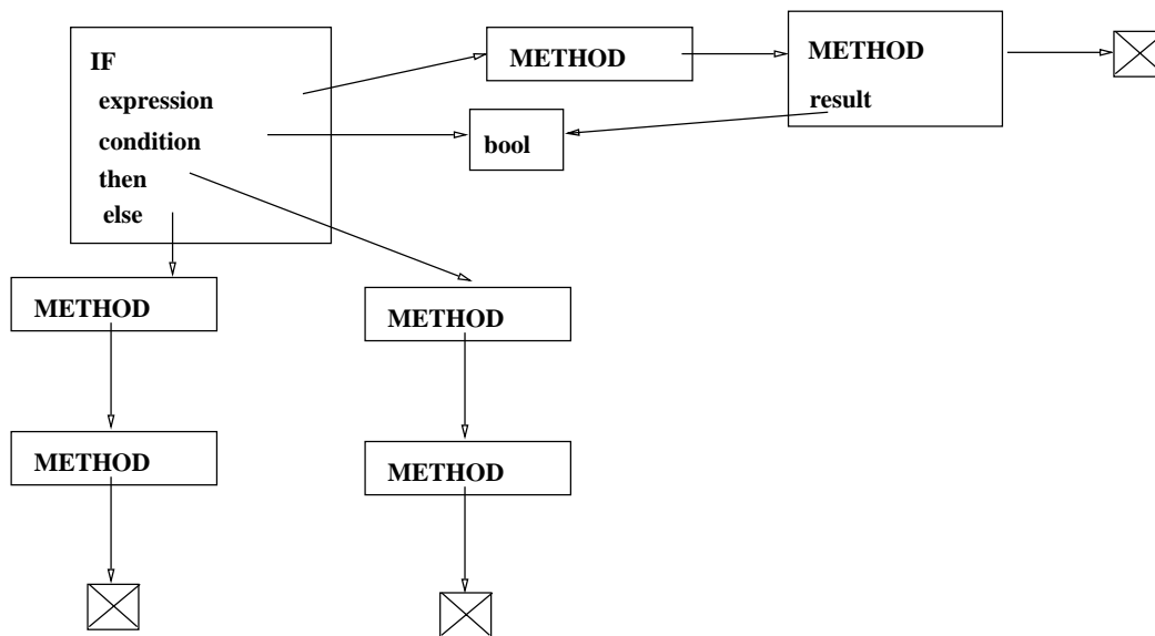
Figure 6-4: If Node
