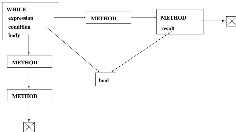
Figure 6-3: While Node
