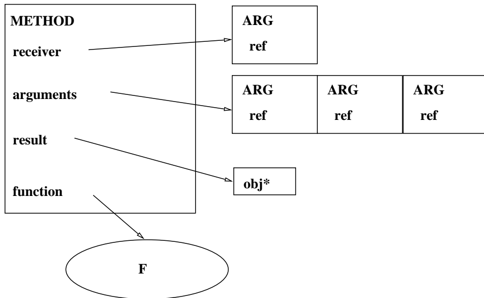
Figure 6-2: Method Node
