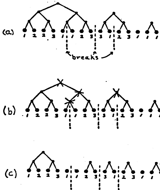
Figure 3. An illustration of the procedure described in Lemma 3.
