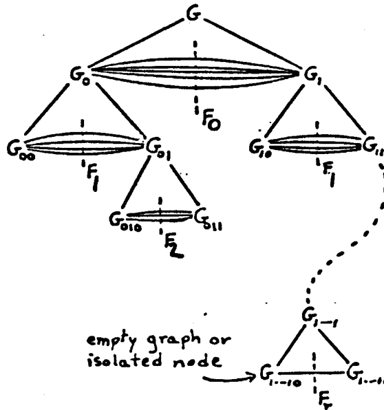
Figure 4. An (F_0, F_1, \dots, F_r) -decomposition tree.
