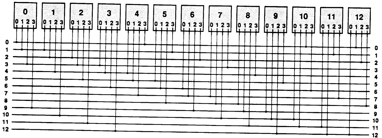
Figure 2-1: A cyclic shifter on 13 chips that uses 13 busses. Each chip has 4 pins, and each bus has 4 chips connected to it. This cyclic shifter is based on the difference cover \{0, 1, 3, 9\} for \mathbf{Z}_{13} .
