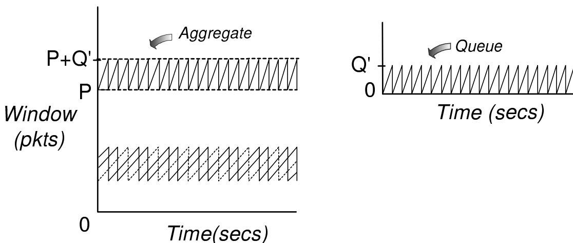
Figure 4-2: Desired dropping behavior for new RED signal
