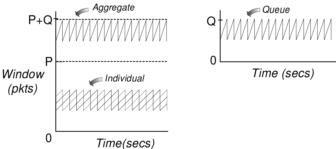
Figure 4-1: Windows of three TCP flows in congestion avoidance
