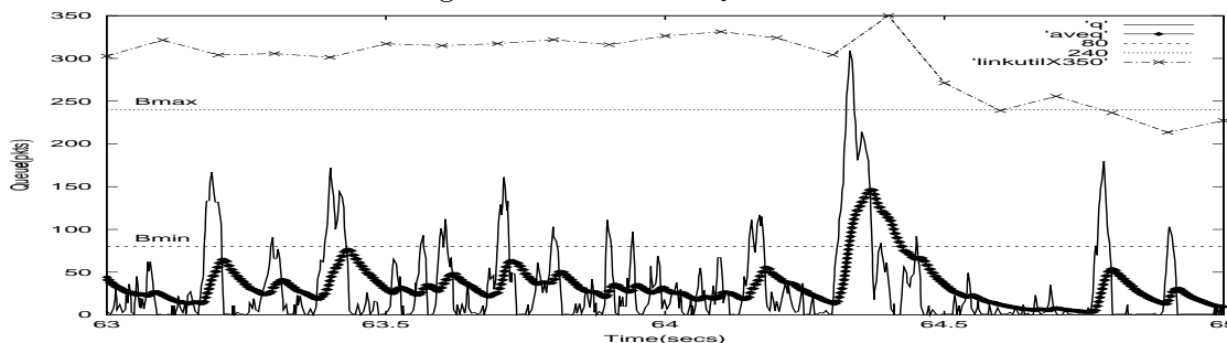
Figure 5-3: Two-way traffic
