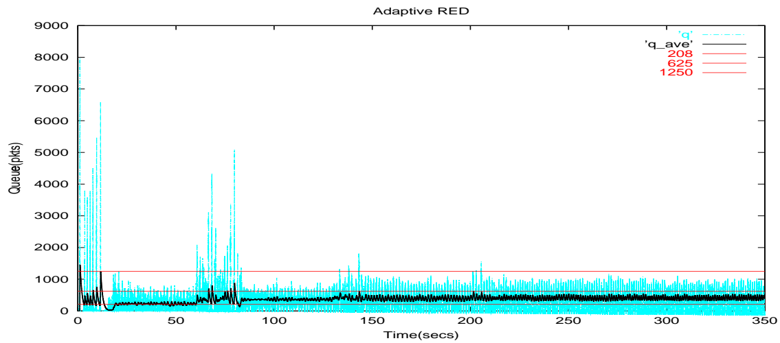
Figure 6-5: Adaptive RED Queue behavior with large N
