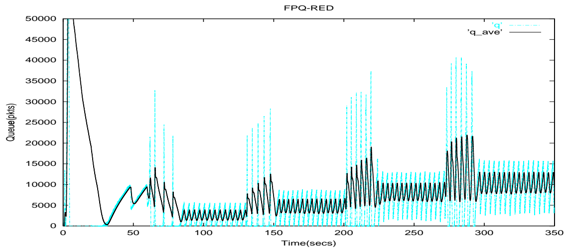
Figure 6-8: FPQ-RED Queue behavior with large N
