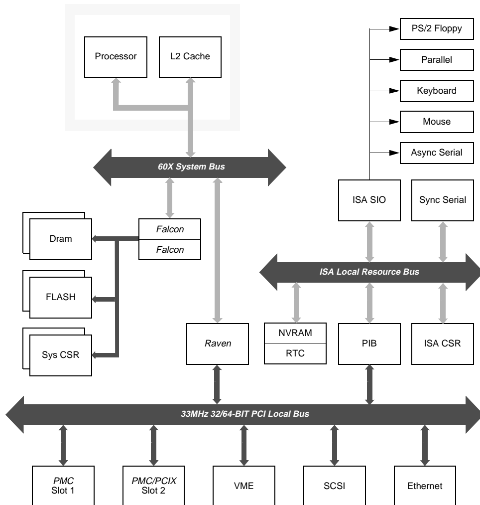
Figure 3-1 is a block diagram of the MVME2603/2604's overall architecture.
