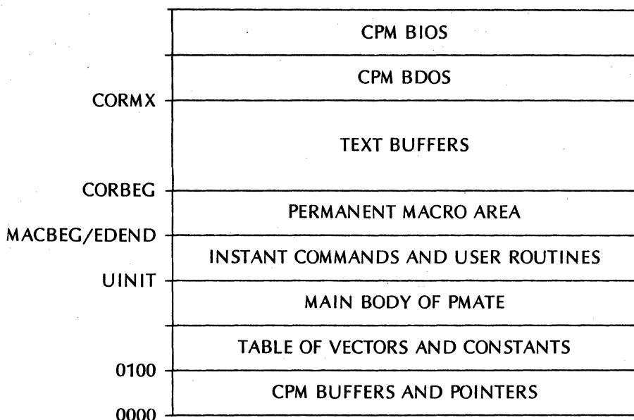
Fig 6-1. PMATE memory allocation.
