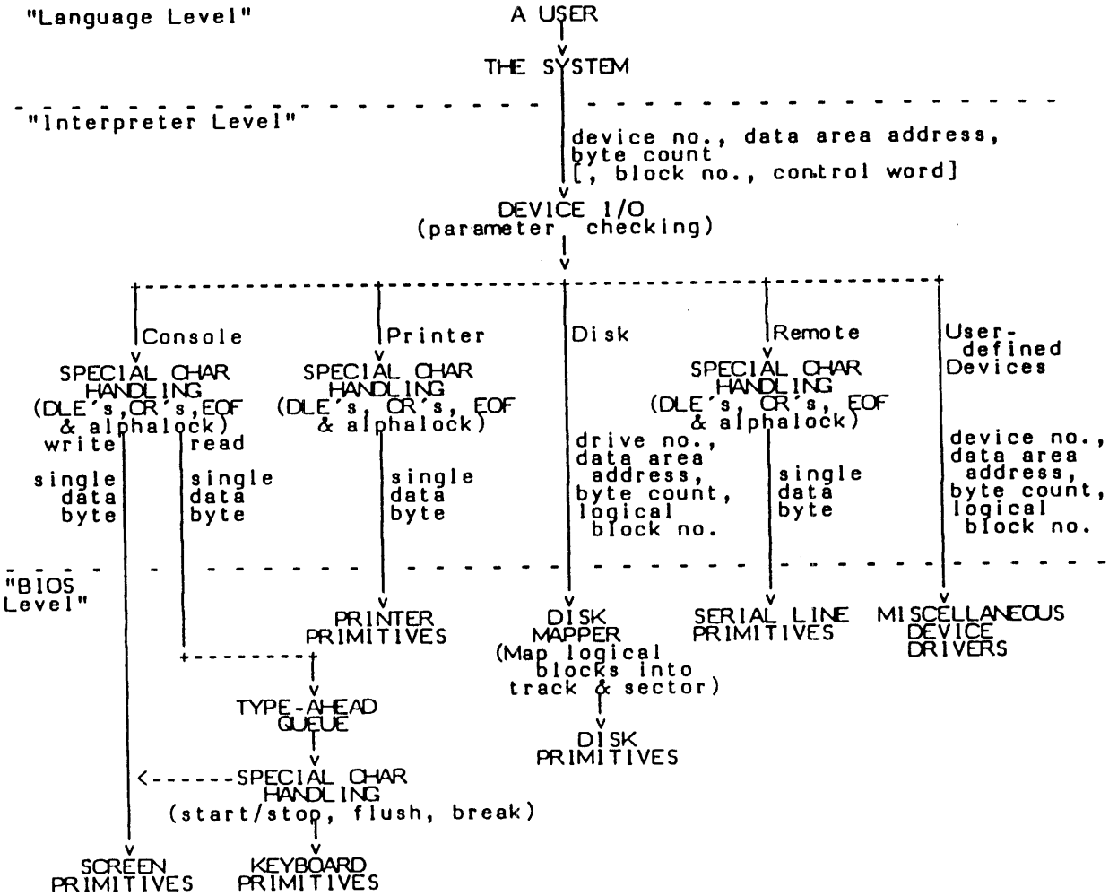
Diagram 1.0 ---- I/O Subsystem Hierarchy
