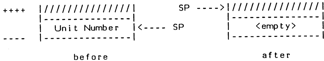
Diagram 3.2 - Stack state before and after UNITWAIT and UNITCLEAR
