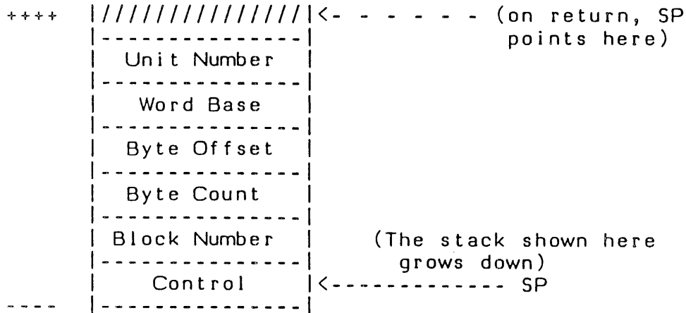
Diagram 3.0 - Stack state on entering UNITREAD or UNITWRITE
