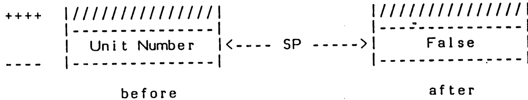
Diagram 3.1 - Stack state before and after UNITBUSY
