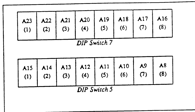
Figure 2-3 Address Switches for the 24-Bit Multibus Memory Space
