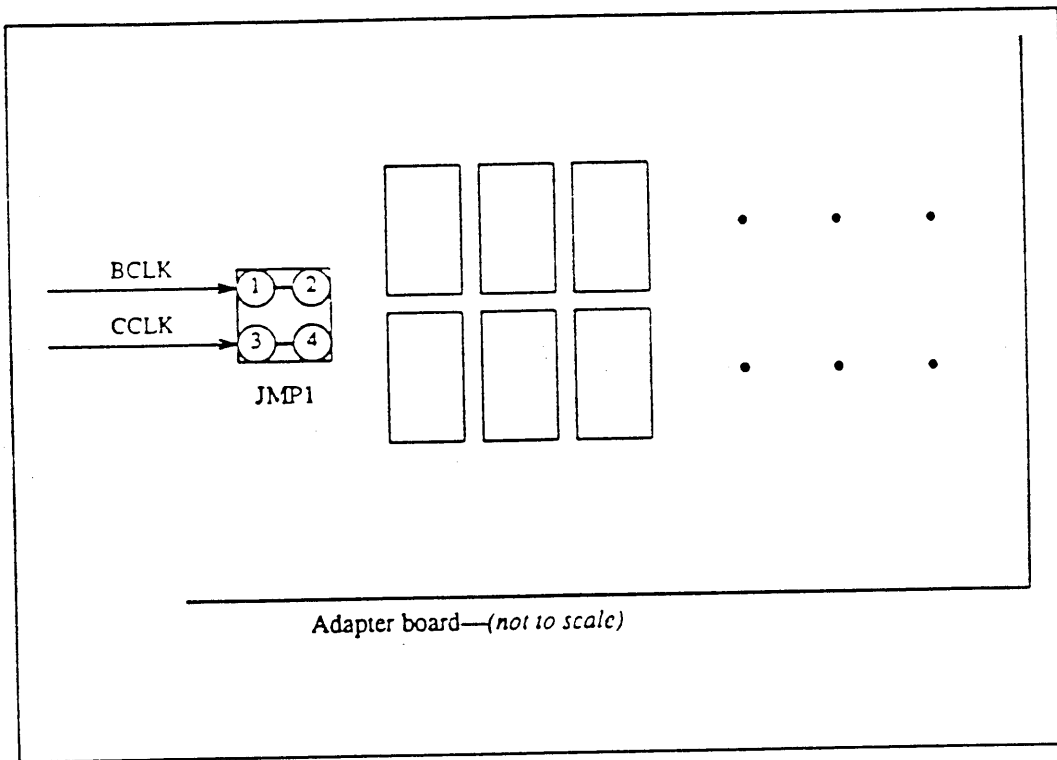
Figure 2-16 BCLK and CCLK Jumper, JMP1
