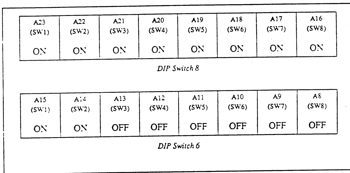
Figure 2-5 Memory Space Block Size Switches for a 16 Kbyte Block
