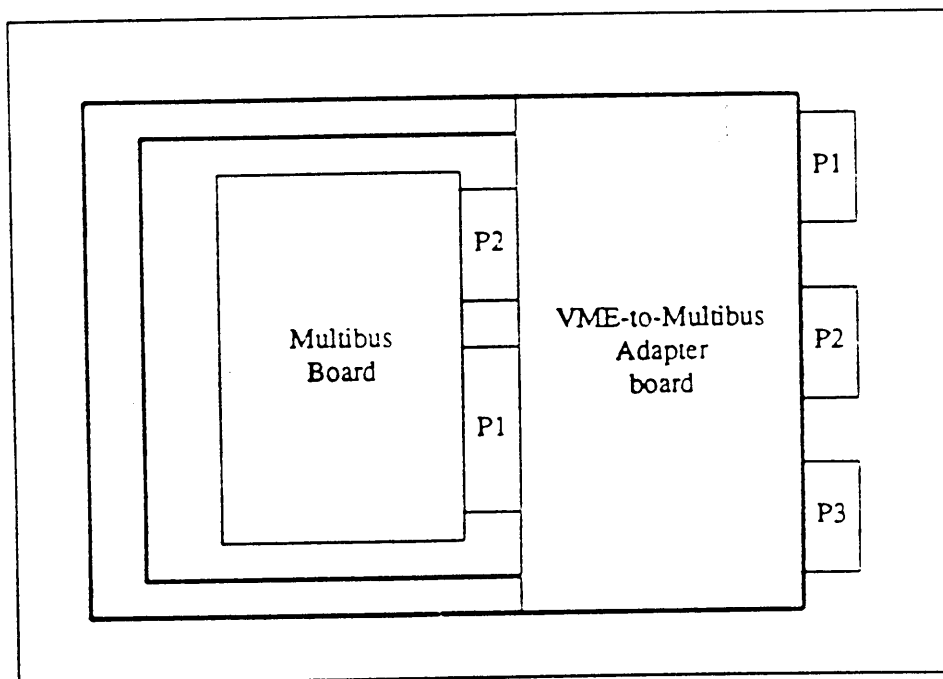
Figure 1-1 VME-to-Multibus Adapter Board
