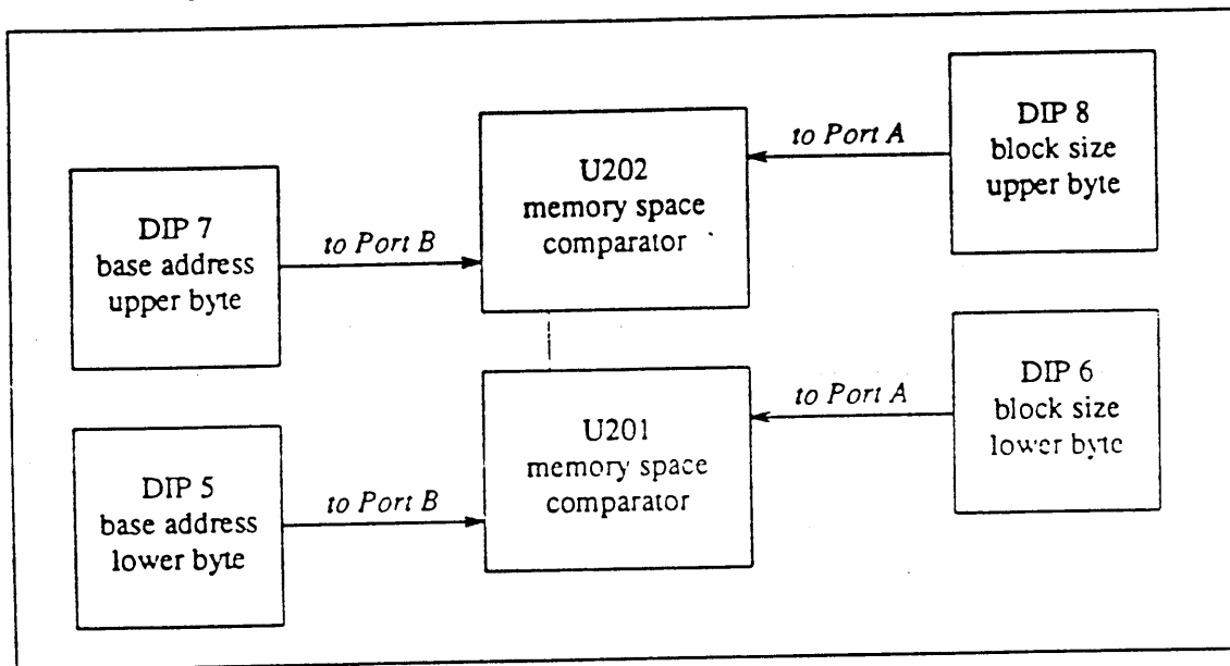
Figure 3-2 Memory Space Switches and Comparators
