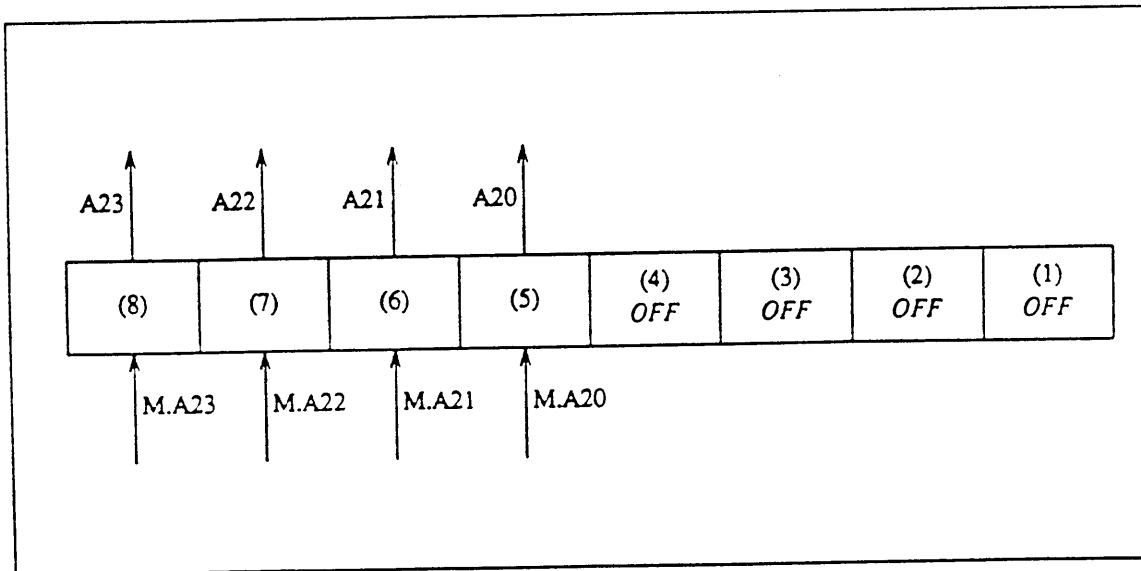
Figure 2-10 DIP Switch 11, Sections 5-8
