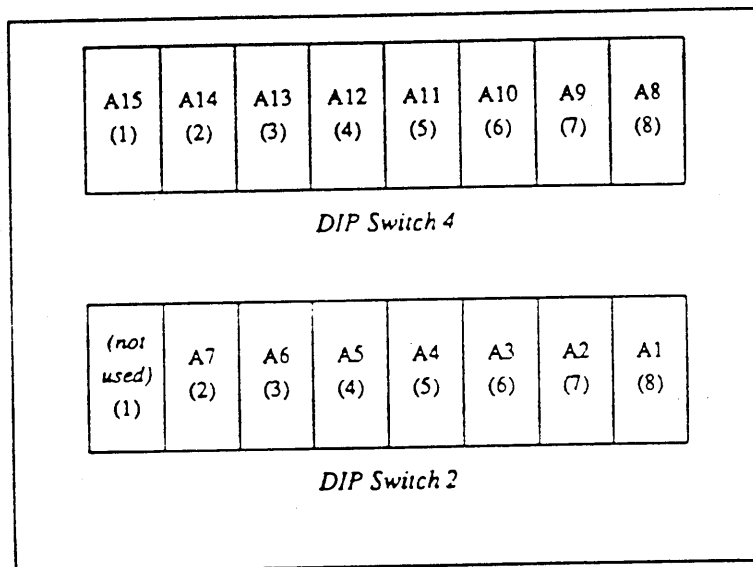
Figure 2-9 Block-Size Switches for the Multibus I/O Space
