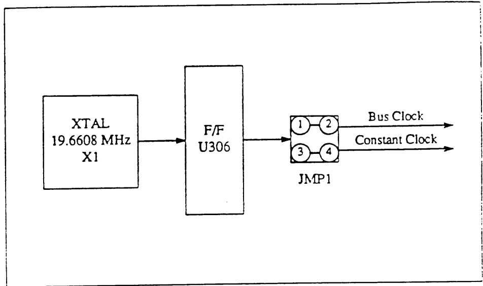
Figure 3-8 BCLK and CCLK Circuitry
