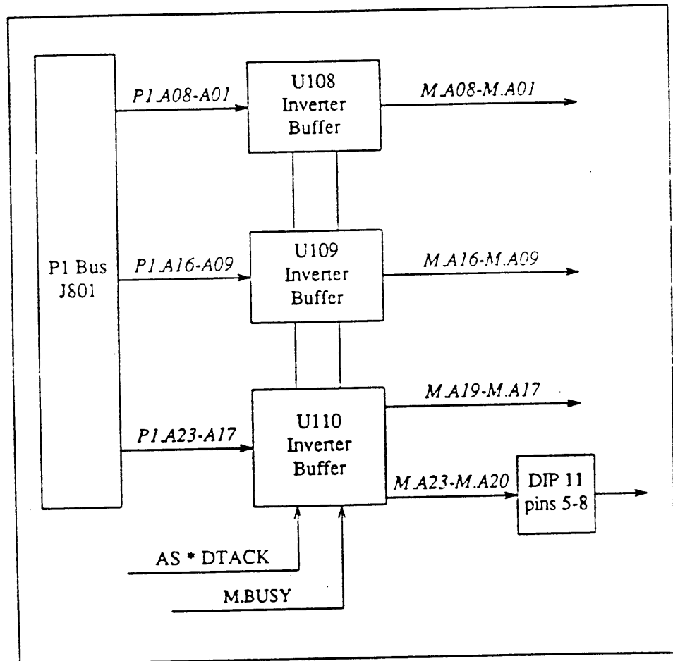
Figure 3-5 Address Signal Flow: VMEbus to Multibus Board
