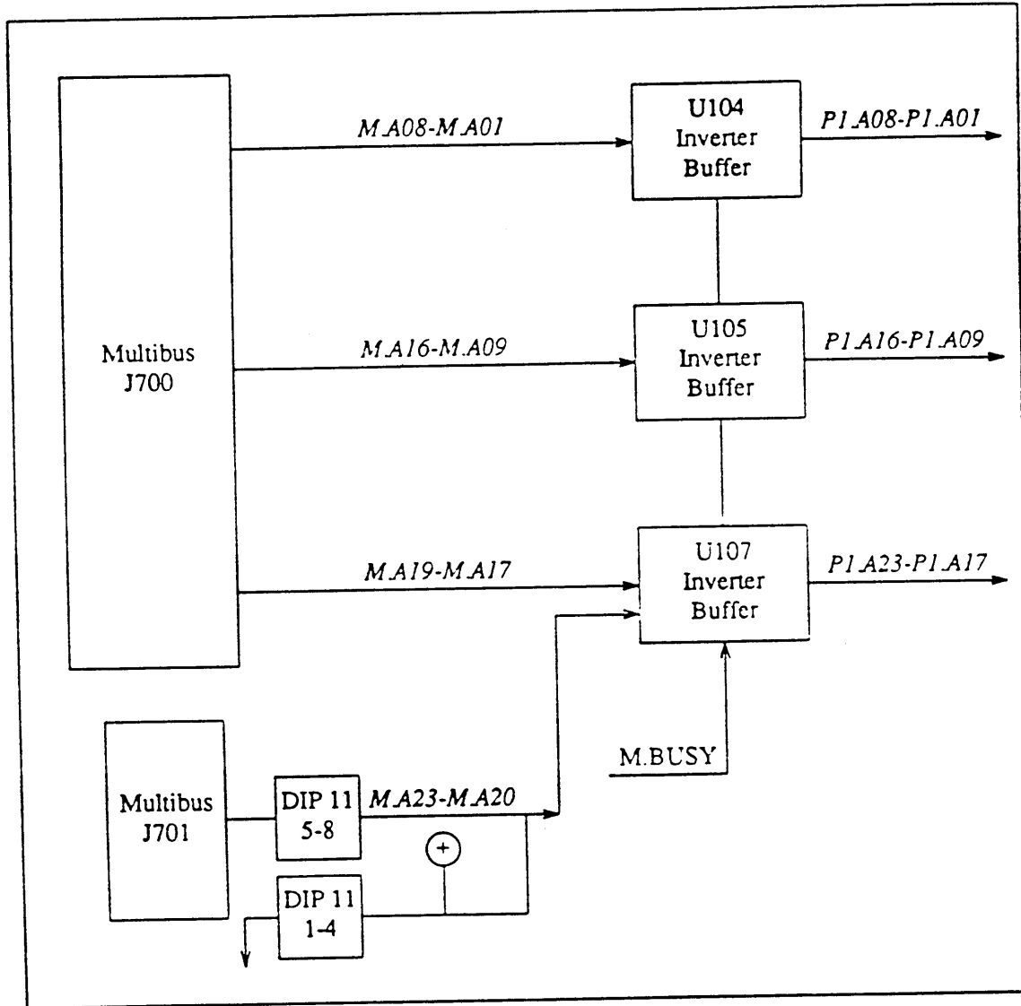
Figure 3-6 Address Signal Flow: Multibus Board to VMEbus
