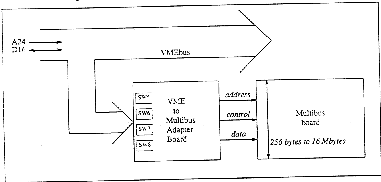
Figure 2-2 Multibus Memory Address Decoding
