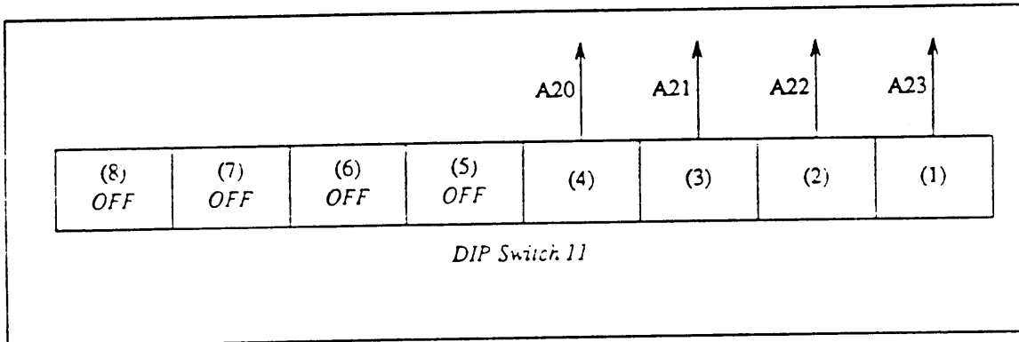
Figure 2-13 DIP Switch 11, Sections 1-4
