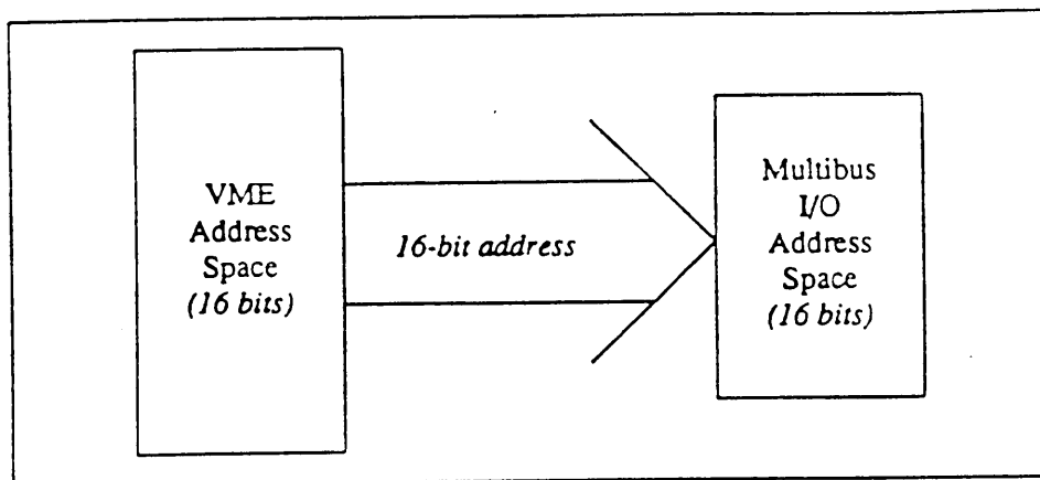
Figure 3-3 VME and Multibus I/O Address Space
