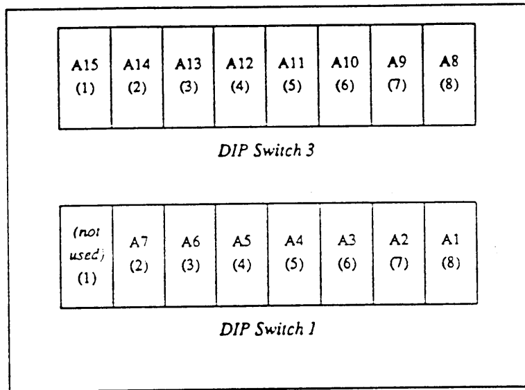
Figure 2-8 Address Switches for the Multibus I/O Space
