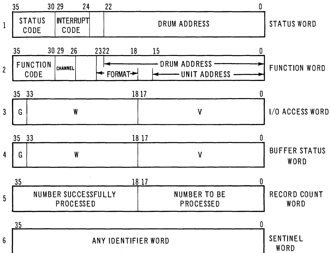
FIGURE 7: I/O EXECUTION PACKET
