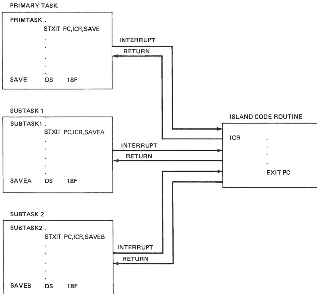
Figure 2-11. Example of Common Program Check Island Code for All Tasks in a Job Step
