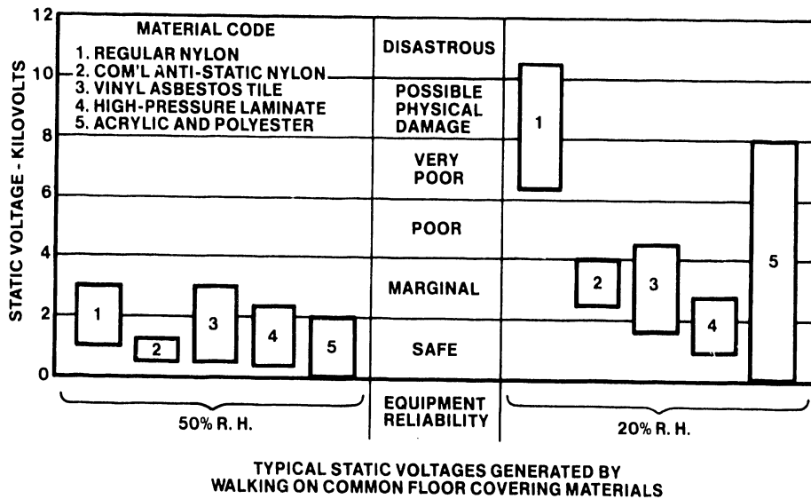
FIGURE 2-1 STATIC POTENTIAL OF COMMON FLOOR COVERINGS
