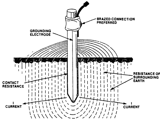
FIGURE 4-5 EARTH GROUND STAKE (Ground Rod)
