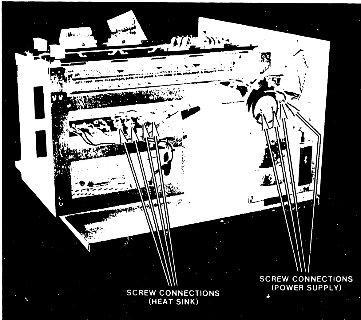
Figure 4-12. Wiring Connections
