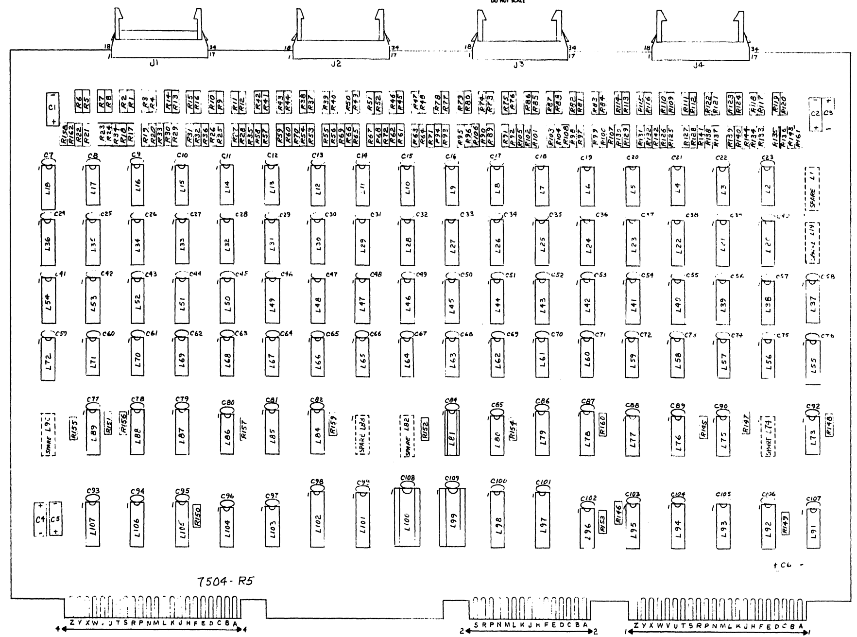
COMPONENT LAYOUT
