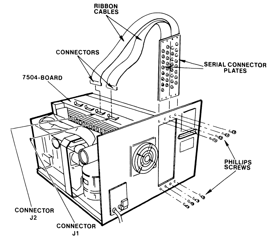
Figure 5-19. Removing/Replacing the Serial Connector Plate Assembly
