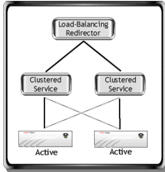
Figure 26: Load-balanced cluster
