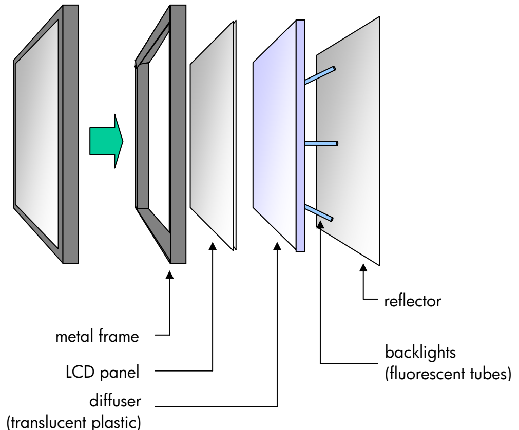
Figure 1—LCD Monitor Components
