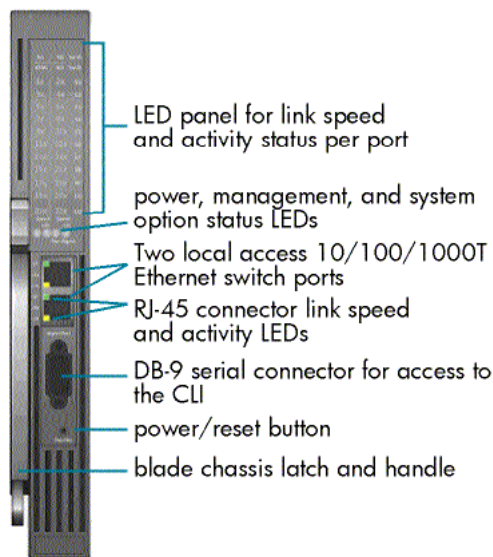
Figure 7. ProLiant BL p-Class GbE2 Interconnect Switch front panel
