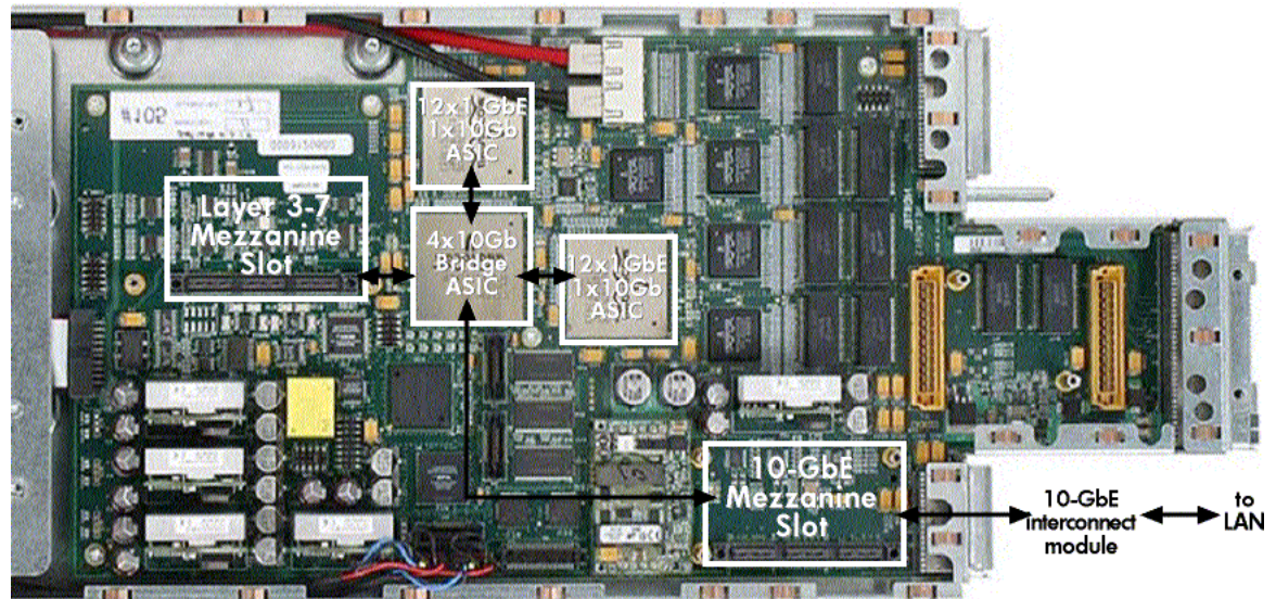
Figure 3. ProLiant BL p-Class GbE2 Interconnect Switch 10 gigabit fabric
