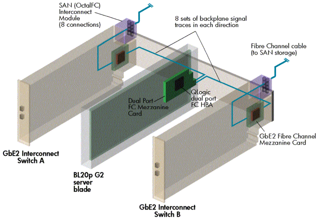
Figure 5. BL20p G2 Fibre Channel signal routing with the GbE2 Interconnect Switch
