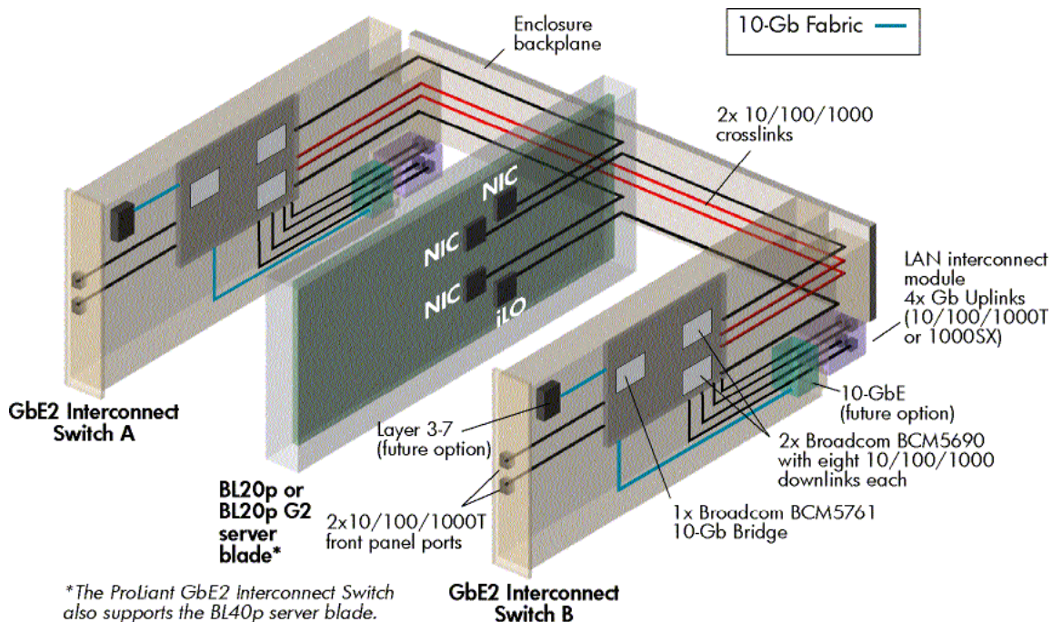
Figure 2. ProLiant BL p-Class GbE2 Interconnect Kit architecture
