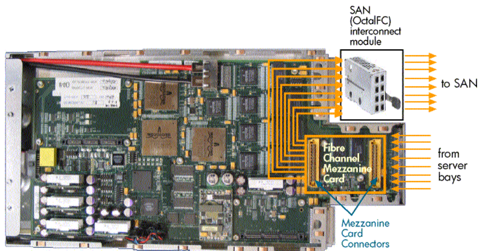
Figure 4. GbE2 Interconnect Switch with GbE2 Storage Connectivity Kit
