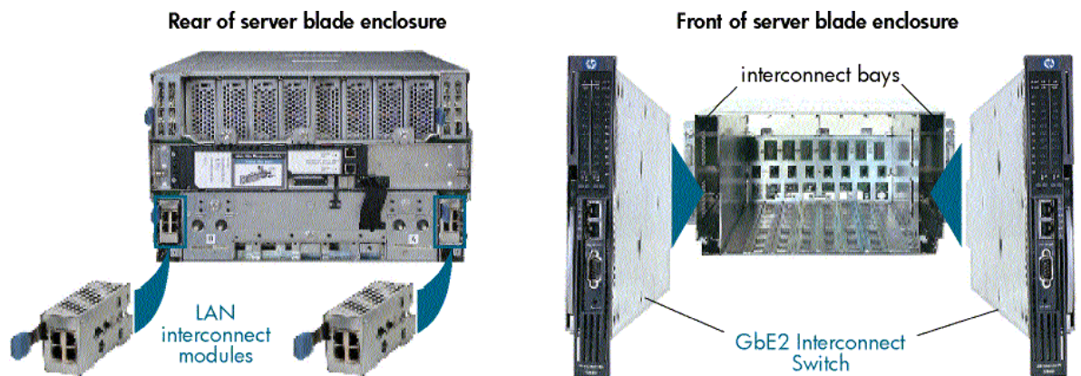
Figure 1. Installation of LAN interconnect modules and GbE2 Interconnect Switches
