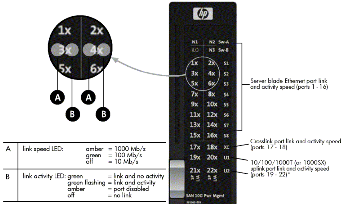
Figure 10. Front port LED panel for ProLiant BL p-Class GbE2 Interconnect Switch
