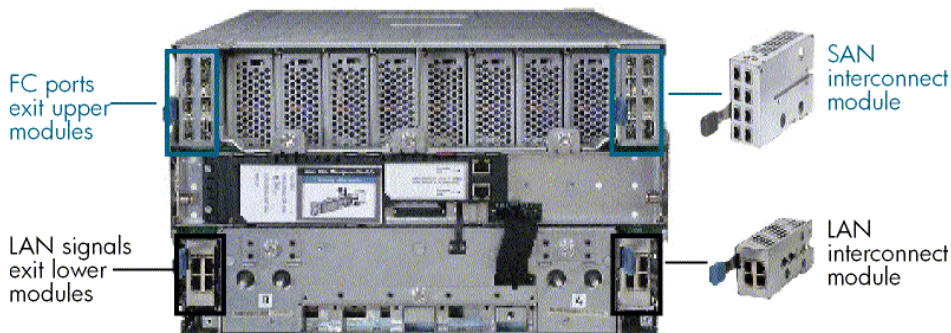
Figure 6. Rear of server blade enclosure with both SAN and LAN interconnect modules installed
