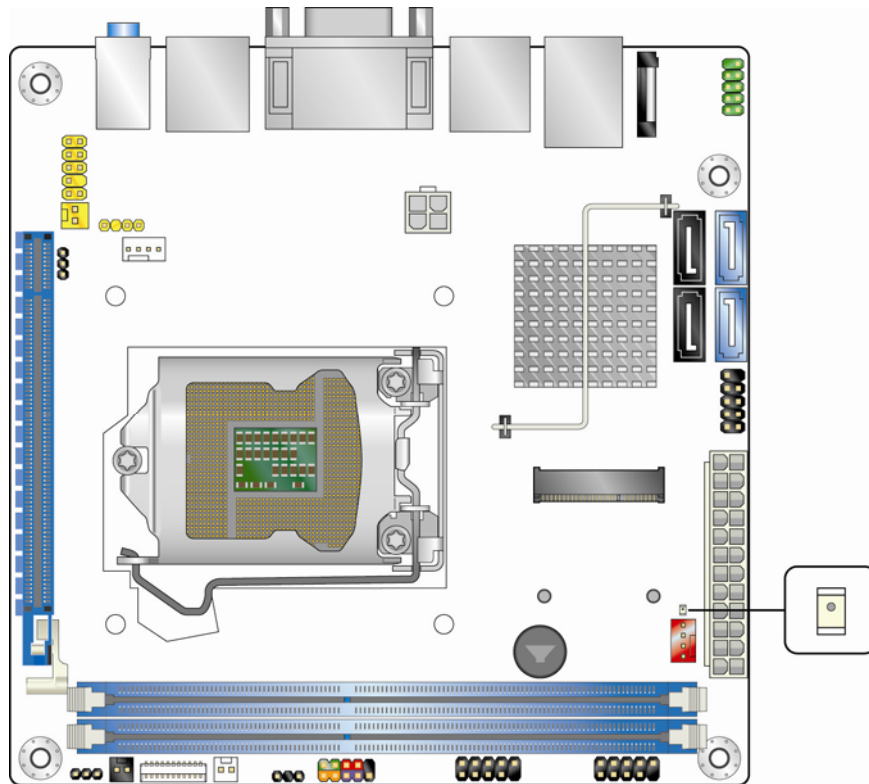
Figure 7. Location of the Standby Power LED (Green)
