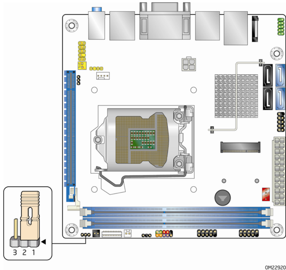
Figure 13. Location of the Jumper Block
