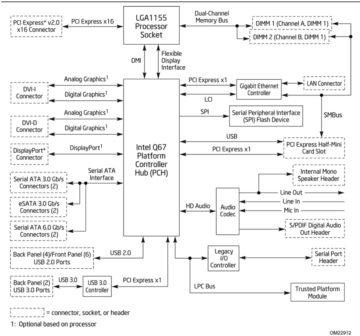
Figure 2. Block Diagram
