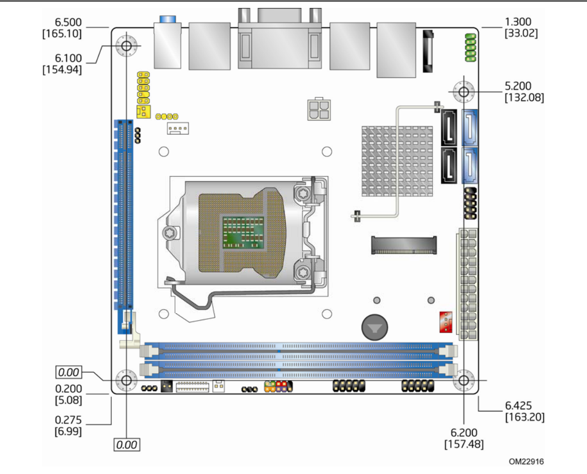
Figure 15. Board Dimensions
