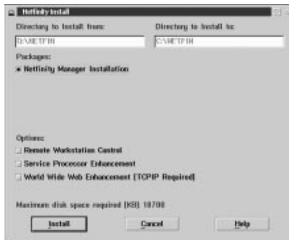
Figure 1. The Netfinity Manager Installation Program
